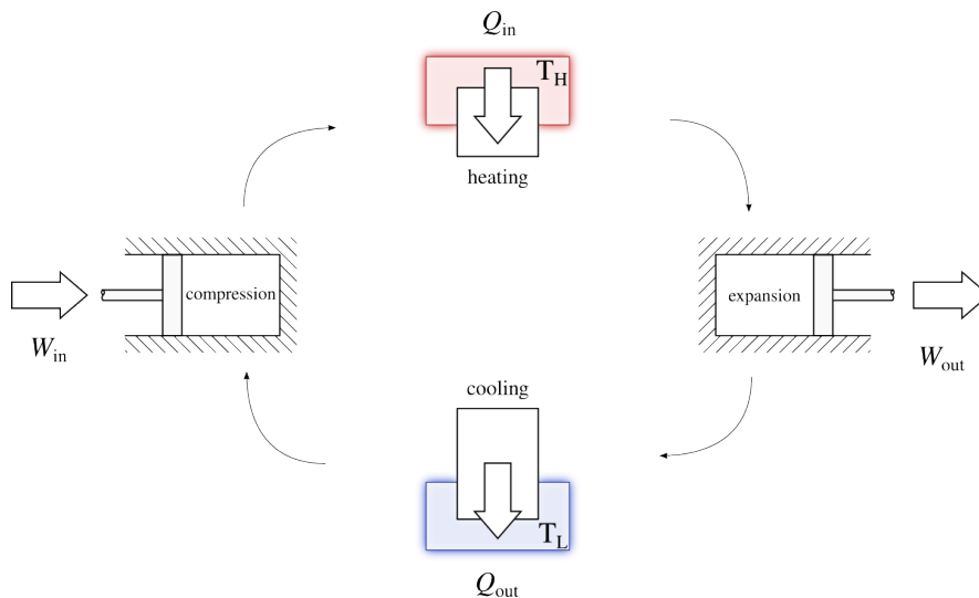
Figure 6.3: Engine thermodynamic cycle carried out by separating the stages in time (rather than in space as shown in figure 6.2). The fluid is heated by a high-temperature heat source T_H . The net work W_{net} = W_{in} + W_{out} is negative.
