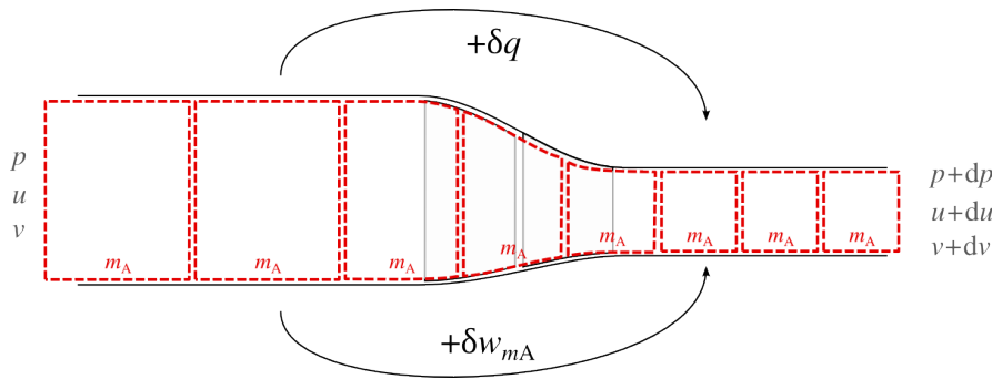
Figure 3.4: A fixed mass quantity m_A flows from left to right through a compressor. It is compressed: its properties change from p and v to p + dp and v + dv . If we consider the point of view of a closed system in transit, the work transfer is \delta w_{m_A} = -p dv .
