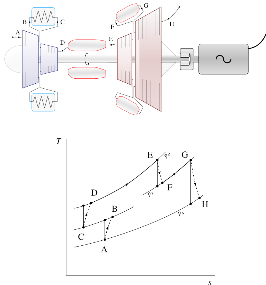
Figure 10.22: A turboshaft generator with intercooler and reheat system (schematic and temperature-entropy diagram).
