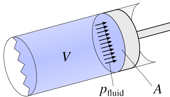
Figure 2.8: When the piston motion is infinitely slow, the fluid behaves like a spring being compressed.
