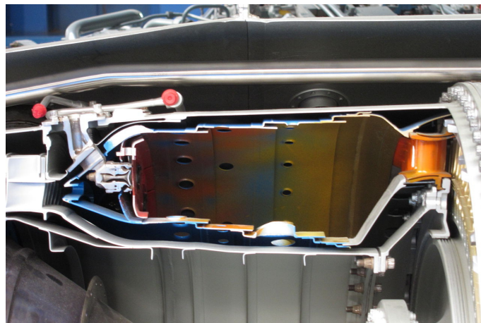
Figure 10.10: Section of an annular combustion chamber in which the flow was from left to right. The photo shows a section of a Rolls-Royce Turboméca Adour , a small turbofan engine designed in 1968.
