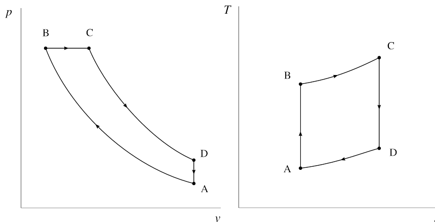
Figure 10.4: Theoretical Diesel cycle represented on pressure-volume and temperature-entropy diagrams. These diagrams depict the ideal path, without compression or expansion irreversibilities.
