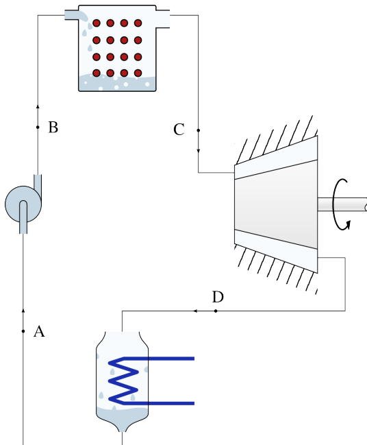
Figure 1.8: Simplified diagram of the water circuit inside a steam power plant. The water follows a complete cycle through four processes.
