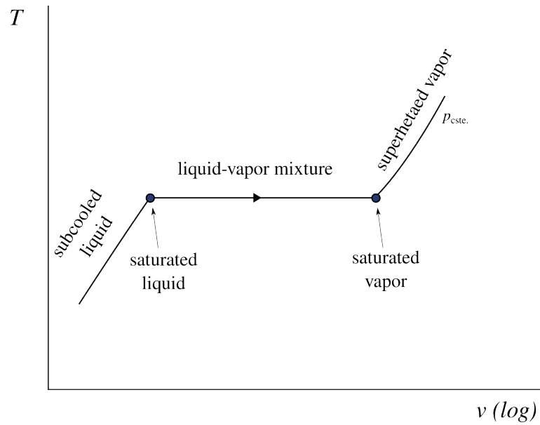
Figure 5.5: Vocabulary: states of the water during a process at constant pressure.
