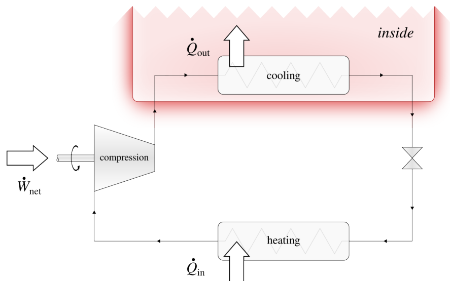
Figure 6.8: Arrangement of a heat pump. The machine is configured to reject heat inside (where the temperature is higher) which it extracts from outside (where the temperature is lower).
