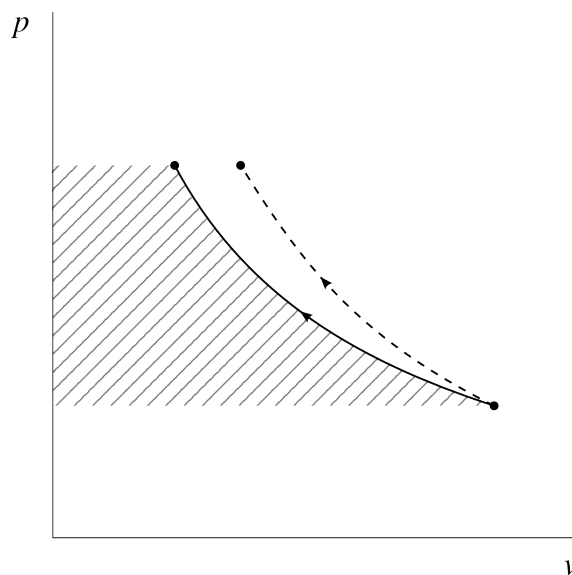
Figure 3.8: Reversible (solid line) and irreversible (dashed line) compressions represented on a pressure-volume diagram. In an open system, work transfers can be visualized with the area to the left of the curve, but only when the processes are reversible.
