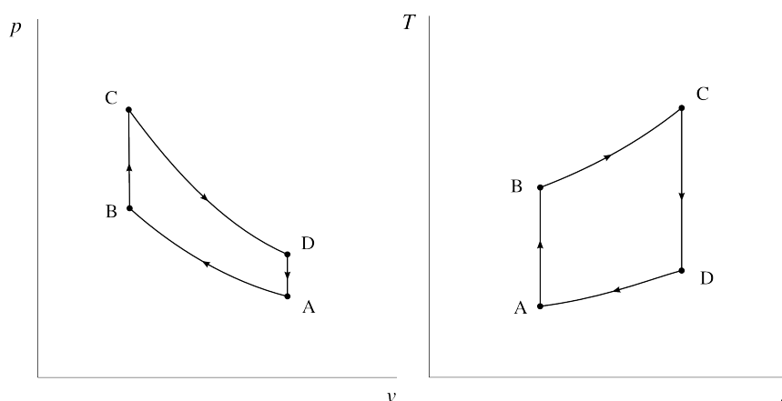
Figure 10.3: Otto's theoretical cycle represented on pressure-volume and temperature-entropy diagrams. These diagrams depict the ideal path, without irreversibilities in the compression or expansion.
