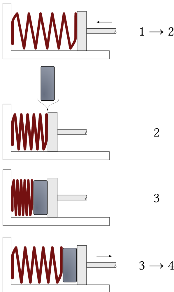
Figure 1.10: Experiment conducted with a powerful spring. The piston compresses the spring from 1 to 2, then the spring pushes back the piston from 3 to 4. On the return path, the force exerted by the spring is greater.
