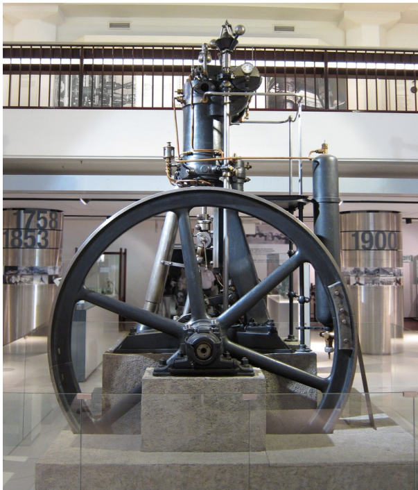
Figure 7.15: Diesel's third prototype, and his first operational engine. The cylinder diameter was 25 cm and the stroke reached 40 cm. It would be tested at the technical university of Munich where it achieved 26.2 % efficiency in 1897. It is exhibited at the Deutsches Museum.
