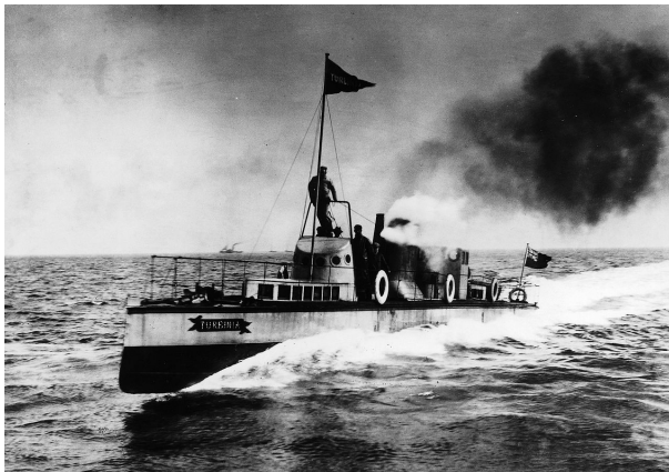
Figure 9.23: The Turbinia , Charles Parsons' yacht used as a demonstrator for his research in maritime propulsion. With its three steam turbines and nine propellers, it reached 60 km/h and allowed its owner to ridicule the Royal Navy during Queen Victoria's jubilee parade in 1897.
