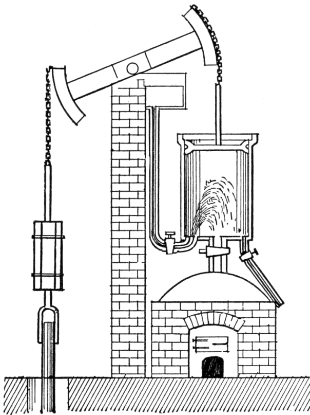
Figure 5.23: Cross-section diagram of one of the first steam engines (Newcomen engine, ~1720). The condensation caused by water injection into the cylinder led to a drop in internal pressure.
