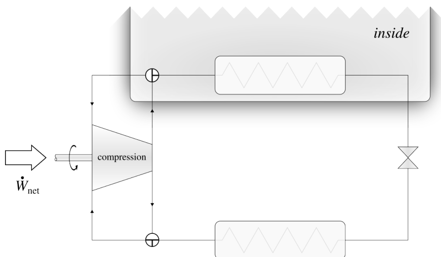
Figure 6.10: Layout of a bidirectional (commonly called “reversible”) air conditioner. By rotating both valves 90 degrees counterclockwise, the function changes from a heat pump to an air conditioner.
