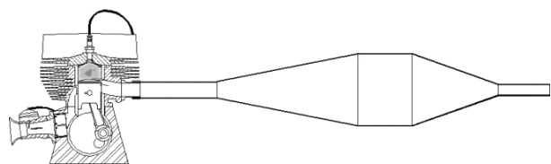
Figure 6.17: Tuned (sometimes called “harmonic”) expansion chamber mounted on a two-stroke engine. Since the flow is unsteady, it is possible to manipulate the pressure exerted by fixed amounts of exhaust gases on the exhaust port when they pass through the chamber. Passing through the expansive part reduces the pressure (thus facilitating scavenging during the piston descent), while passage through the contraction, on the contrary, increases this pressure (thus reducing gas losses during the piston ascent).
