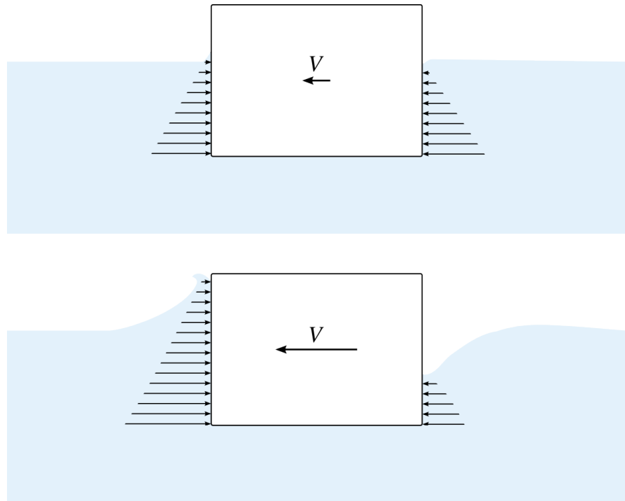
Figure 2.12: A solid object being moved in a water tank, with slow motion (above) and with fast motion (below). During fast motion, the pressure forces aiding the movement are weaker, and the forces opposing the movement are greater. In the limit of infinitely slow motion, these forces are equal.
