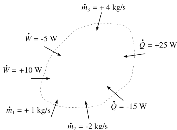
Figure 3.1: Sign conventions for an open system. Inflows are positive, outflows are negative; they are all represented with inward arrows.
