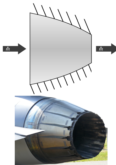
Figure 3.13: Schematic diagram of a nozzle and installation (with variable geometry) on the Pratt & Whitney F100 engine of a Lockheed Martin F-16.
