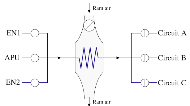
Figure 6.24: Diagram representing the air arriving in the conditioning pack from the engines (EN1 and EN2) or the auxiliary power unit (APU) on the left. This air exits into one of the three circuits A, B, or C after losing heat to the RAM air.
