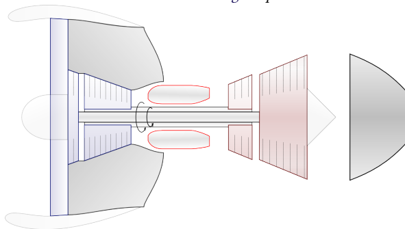
Figure 10.37: Schematic diagram of the arrangement of the General Electric CF6 .
