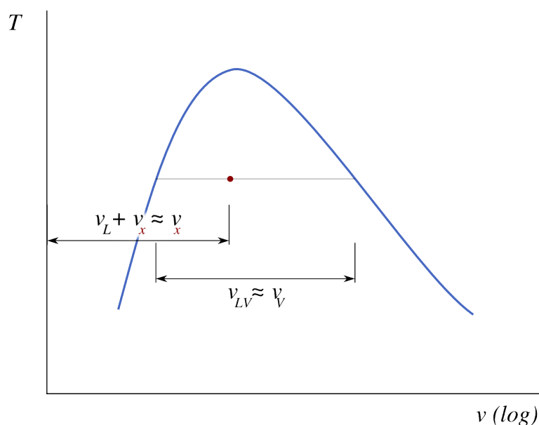
Figure 5.13: Approximations used in calculating the volume occupied by a liquid-vapor mixture. It should be noted that the abscissa scale is logarithmic: v_L is generally several hundred times smaller than v_V , and the approximation is not graphically emphasized.
