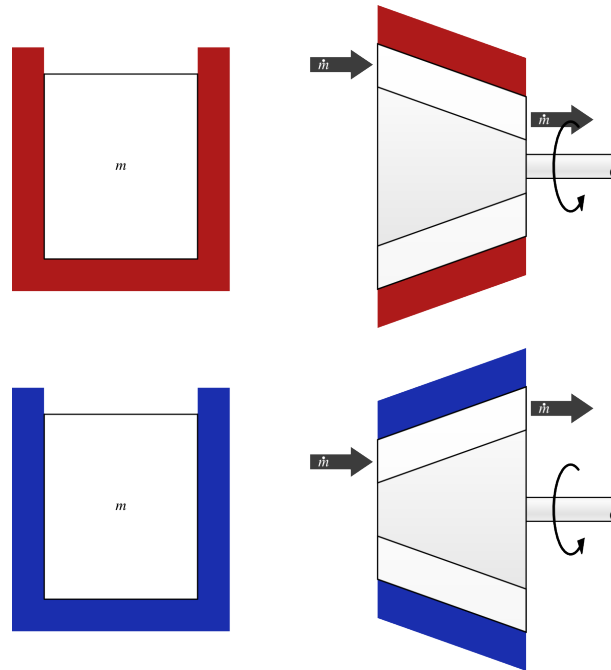
Figure 4.8: A constant-volume (isochoric) process undergone by an ideal gas. In a closed system (left), the volume is fixed and no work is done. In an open system (right), the gas must be compressed while heating and expanded while cooling, to maintain the specific volume constant.
