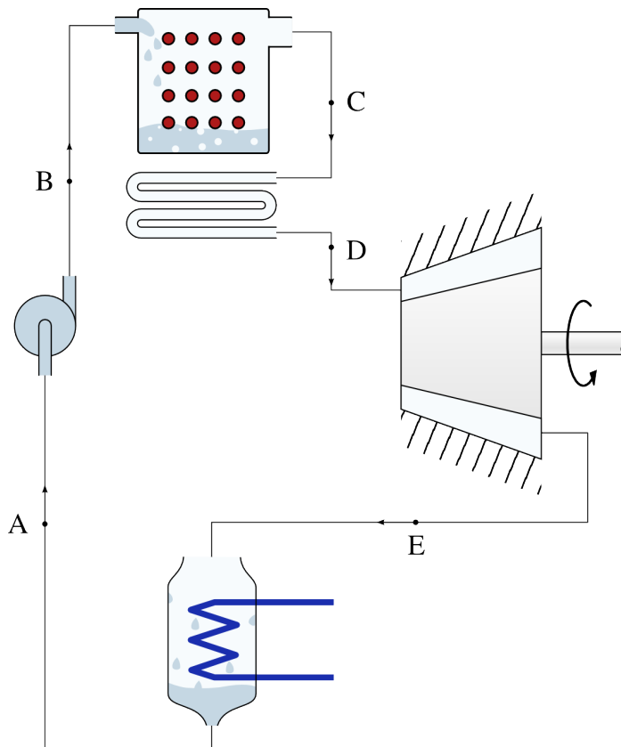
Figure 9.14: Diagram of a steam power plant operating on a superheated Rankine cycle. The water at the outlet of the boiler is heated to a higher temperature (section C → D) before entering the turbine.
