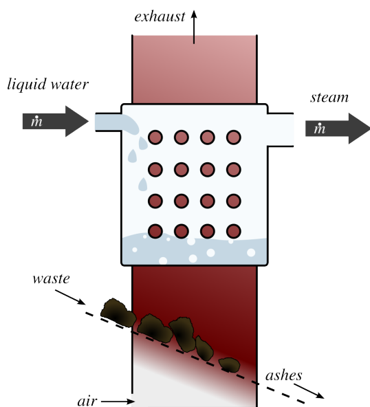
Figure 3.12: Schematic diagram of a boiler operating from the combustion of waste.
