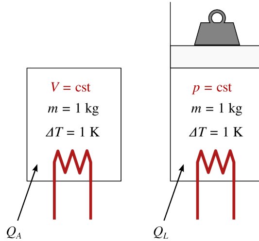
Figure 4.3: Definitions of heat capacities. On the left, the volume is fixed and the specific thermal capacity will be c_v . On the right, the pressure is constant and the capacity will be c_p .
