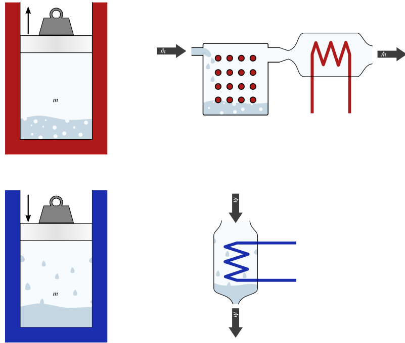
Figure 5.14: Constant-pressure (isobaric) process undergone by a liquid/vapor. In a closed system (on the left), the piston exerts a constant force throughout the process. In an open system (on the right), no work is done.
