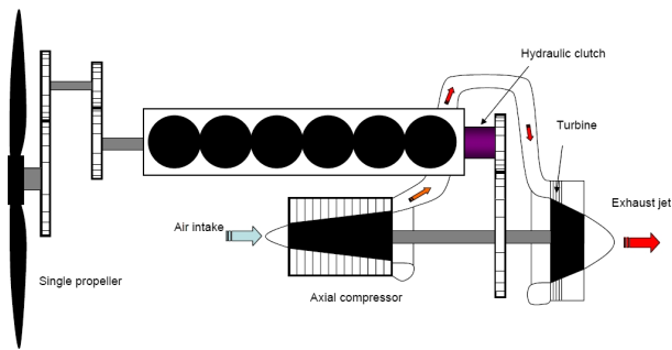
Figure 10.29: Schematic diagram of the thermodynamic circuit of the Napier Nomad II . A variable-ratio mechanical-hydraulic reducer connected the two units, which now drove the same propeller.
