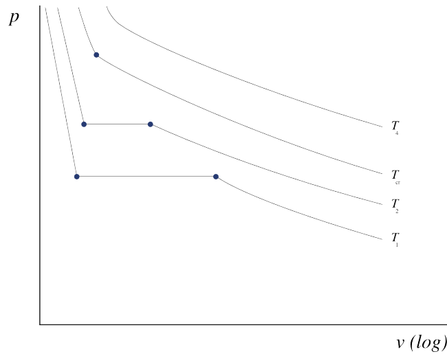
Figure 5.8: Properties of water plotted on a pressure-volume diagram, when maintaining constant temperature by varying the volume.
