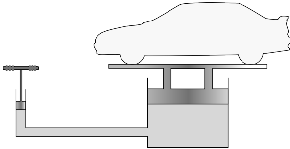
Figure 1.11: Schematic diagram of a hydraulic jack.
