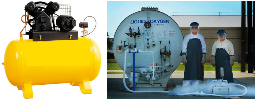
Figure 1.4: Left: when air is compressed in a compressor, air gives heat away through the sides and the fins of the cylinders; and yet, its temperature increases. Right: by contrast, when liquid oxygen is expanded in a valve, liquid oxygen receives heat from the atmosphere (as evidenced by the condensation and frost from atmospheric air on the piping); in spite of this, its temperature drops.
