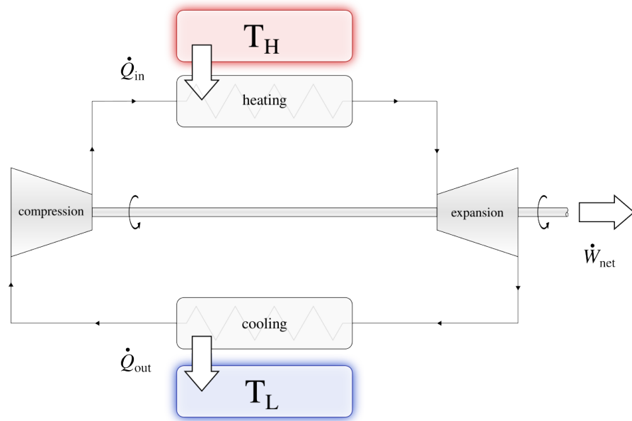
Figure 6.4: An engine thermodynamic cycle in which the compressor and the turbine are mechanically coupled. Since the turbine supplies a power \dot{W}_{out} greater than that absorbed by the compressor ( \dot{W}_{in} ), it is able to not only drive the compressor but also to provide an excess \dot{W}_{net} sent outside of the engine.
