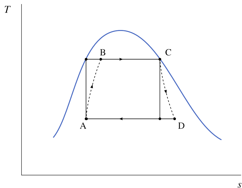
Figure 9.11: Temperature-entropy diagram of a steam power plant operating on a Carnot cycle. The dashed paths represent the real (irreversible) processes of the fluid during compressions and expansions.
