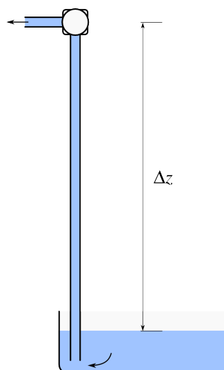
Figure 5.30: Water pumping from a reservoir located below. The first observation of the height limit calculated in this problem was made in 1630 by Giovanni Battista Baliani.
