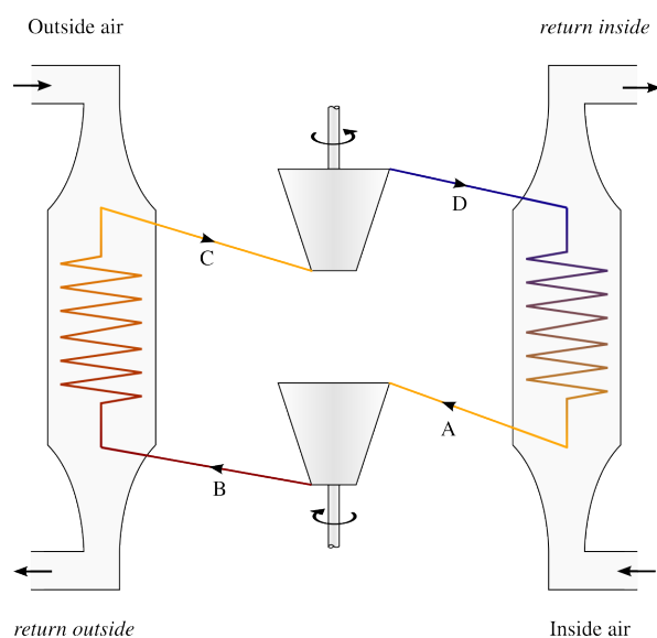
Figure 6.22: Schematic diagram of an air conditioner. The air in the air conditioner circuit circulates in a steady flow ( A \rightarrow B \rightarrow C \rightarrow D \rightarrow A ), without ever leaving the machine.
