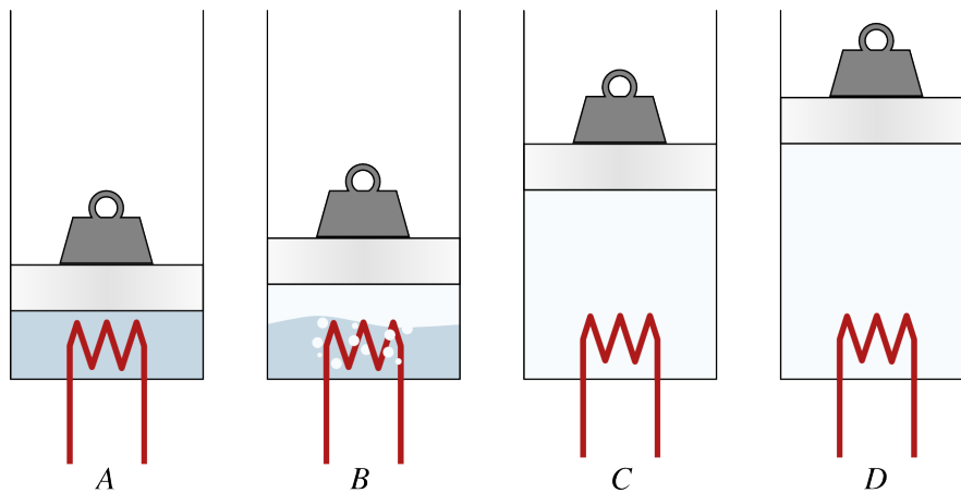
Figure 5.4: Heating of a fixed quantity of water at constant pressure. A: subcooled liquid; B: liquid-vapor mixture; C: saturated vapor; D: superheated vapor.
