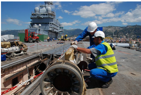
Figure 5.33: Piston of a steam catapult from the aircraft carrier Charles de Gaulle . Photo CC-BY-SA by Jean-Michel Roche, Netmarine.net
