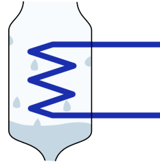
Figure 9.7: Schematic representation of a condenser. Water from the thermodynamic cycle enters at the top, in a state close to saturated vapor. It exits at the bottom in the liquid state. The heat extraction is usually ensured by a secondary water circuit (illustrated in dark blue) which is in contact with the atmosphere.
