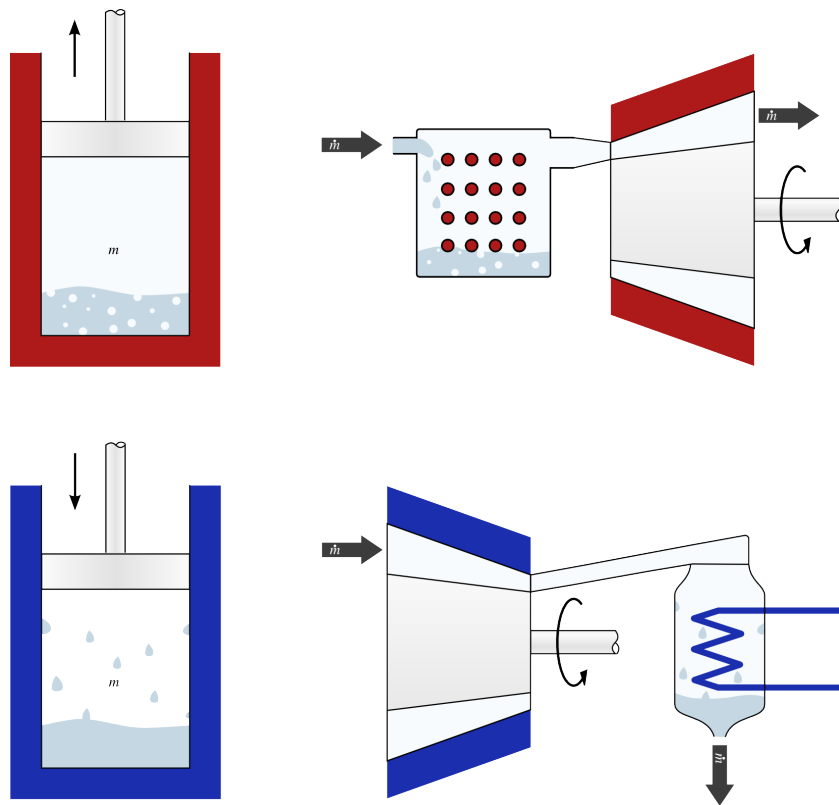
Figure 5.18: A constant-temperature (isothermal) process undergone by a liquid-vapor. In a closed system (left), the gas is allowed to do work on a piston while being heated, and conversely, work is done on it when cooling. In an open system (right), the same manipulations are carried out continuously.
