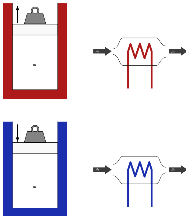
Figure 4.6: A constant-pressure (isobaric) process undergone by an ideal gas. In a closed system (left), the piston exerts a constant force throughout the process. In an open system (right), no work is done.
