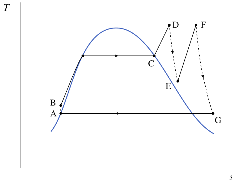
Figure 9.17: Temperature-entropy diagram of a steam power plant operating on a reheated Rankine cycle.
