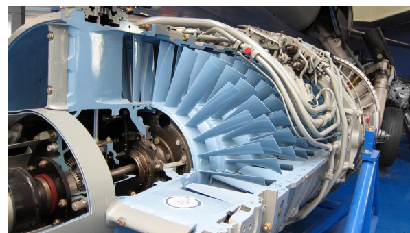
Figure 4.20: Compressor of a disassembled SNECMA Atar turbojet engine (1948). Air flows from the left to the center of the image.
