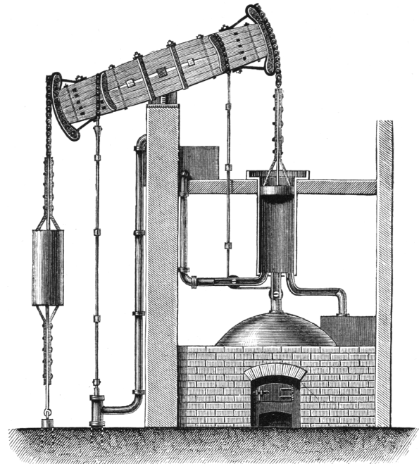
Figure 5.31: The ingenious atmospheric engine by Newcomen, the first true success in steam power.
