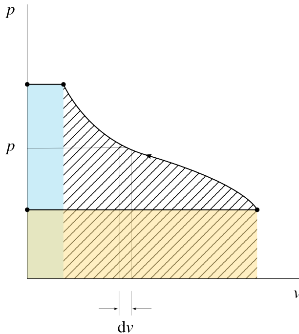
Figure 3.6: Work received by an open system crossed by a fluid, during a slow process.
