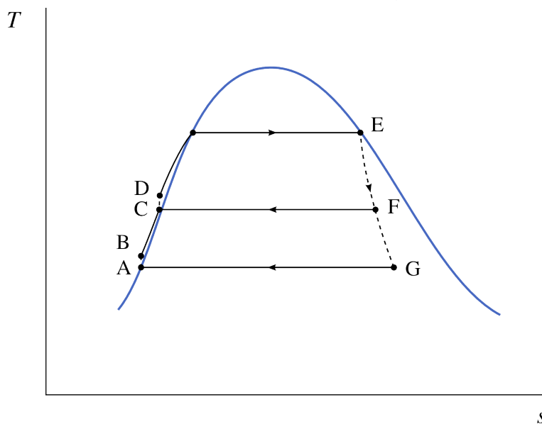
Figure 9.21: Temperature-entropy diagram of a power plant with steam bleed.
