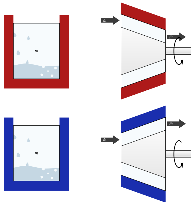
Figure 5.16: A constant-volume (isochoric) process undergone by a liquid-vapor. In a closed system (left), the volume is fixed and no work is done. In an open system (right), the fluid must be compressed while being heated and expanded while being cooled, in order to maintain constant specific volume.
