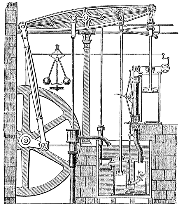
Figure 5.24: The Boulton & Watt engine with separate condensation and double-acting piston.
