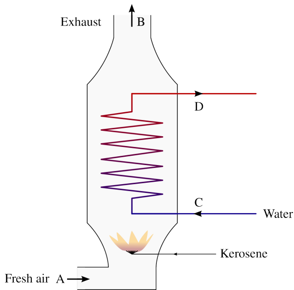
Figure 1.13: Schematic diagram of a boiler used for heating a building. The water ( C \rightarrow D ) enters from the right and is heated by the air ( A \rightarrow B ) mixed with kerosene.
