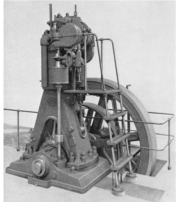
Figure 4.18: Diesel Engine from 1898, manufactured under license by Sulzer in Switzerland
