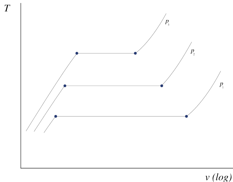
Figure 5.6: Properties of water plotted on a temperature-volume diagram, when conducting the experiment described in figure 5.4 at different pressures. It can be observed that the higher the pressure, the smaller the boiling range becomes.
