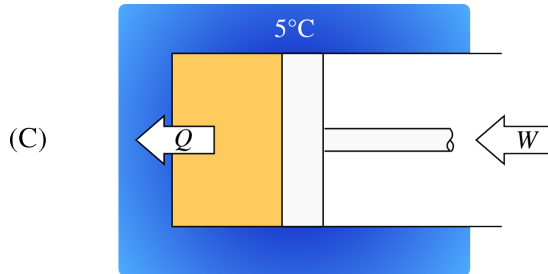
Figure 7.2: The inevitable cooling of the engine. The only way to return the fluid to its initial state (A) in the experiment in figure 7.1 is by extracting heat from it, which can only be done with a “heat sink” at a lower temperature. The heat and work transfers here are smaller than on the outward journey, but both are non-zero.
