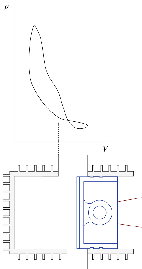
Figure 6.16: Schematic pressure-volume diagram of the cylinder of a two-stroke engine with crankcase intake. It is left to the student to determine which of the two ports (high or low) corresponds to intake and exhaust in the cylinder.
