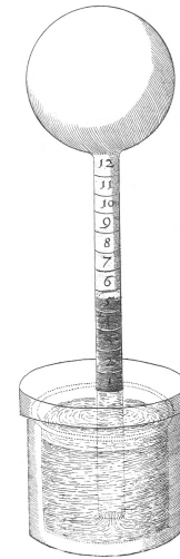
Figure 1.5: An air thermometer from the early 17 th century. The ball was filled with air whose volume varies with its temperature, pushing the water from the reservoir below whose surface is at atmospheric pressure. The liquid could be colored, and its changes height were measured using a scale. Since atmospheric pressure varies with meteorological conditions, it affected the measurements: it was, in a way, a baro-thermometer.
