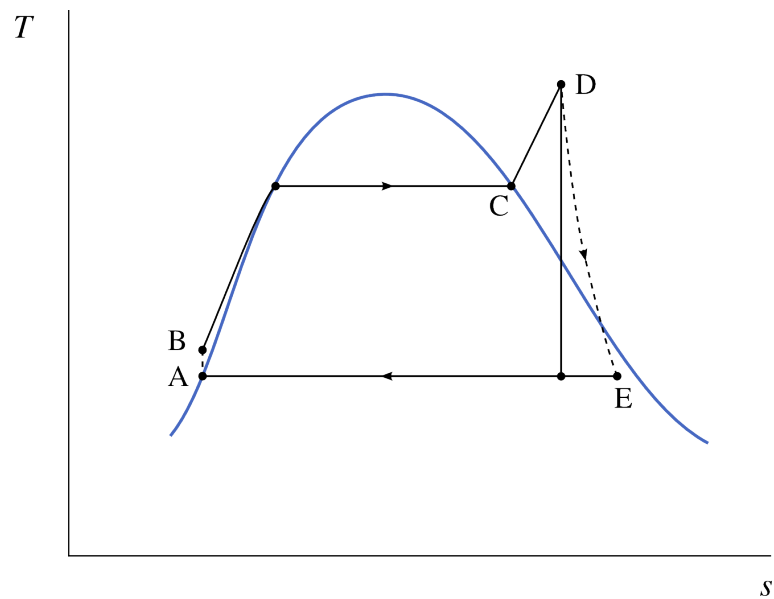
Figure 9.15: Temperature-entropy diagram of a steam power plant operating on a superheated Rankine cycle.
