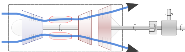
Figure 1.14: A Sikorsky S-76B helicopter, equipped with two P&WC PT-6B turboshaft engines, each with 980 hp. The airflow through the engines is shown in a schematic diagram. We will study these engines in more detail in chapter 10 ( air-based power cycles ).
