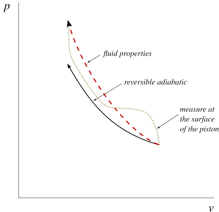
Figure 2.14: Irreversible adiabatic compression on a pressure-volume diagram. We draw the curve with dashes: it is not a continuous series of states because the fluid pressure is not homogeneous during the process. The path the fluid would have followed if the compression had been infinitely slow is represented with a solid line. During compression, the “surplus” of work supplied by the piston is converted into heat, even though the gas is perfectly isolated.
