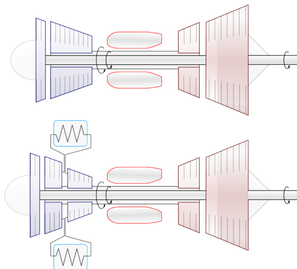
Figure 10.38: Top: schematic diagram of a turboshaft based on the CF6 from which the fan has been removed. Bottom: the same turboshaft engine modified by the addition of an intercooling system.
