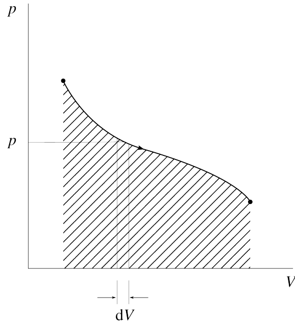
Figure 2.6: Pressure-volume diagram of a closed system modeled by a spring. In the case shown here, the volume is increasing (the piston moves away). The quantity dV remains positive, and the work is negative: the system loses energy by doing work on the piston. This figure represents the same phenomenon as in fig. 1.3 p. 17, using different physical quantities. Diagram CC-0 Olivier Cleynen
