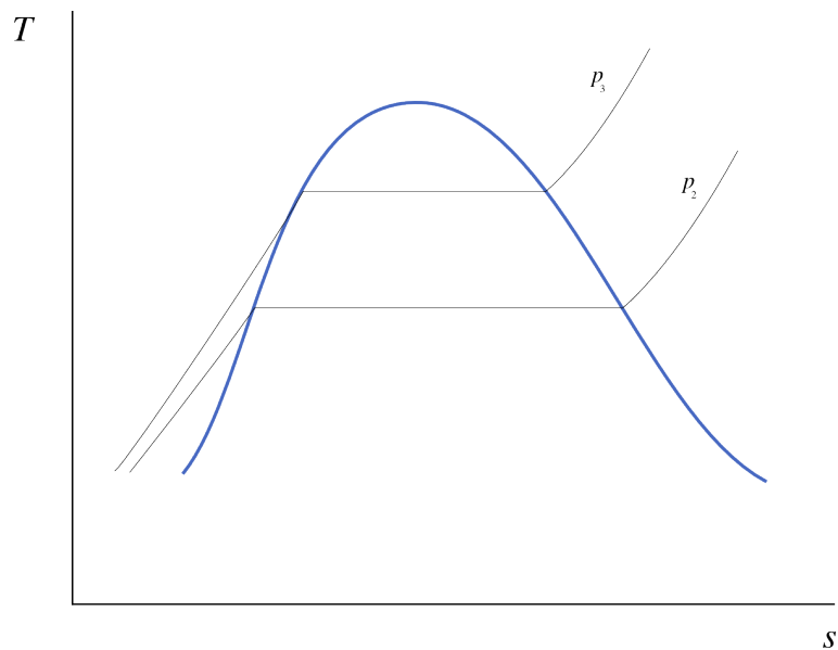
Figure 8.8: Temperature-entropy diagram of a liquid/vapor mixture. This figure closely resembles fig. 5.7 p. 121.
