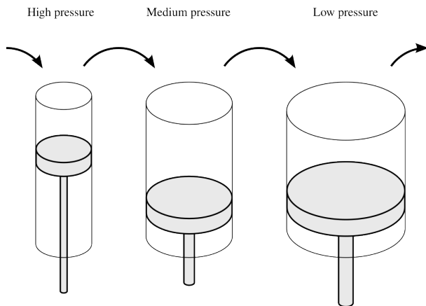
Figure 2.17: Cylinders in series, known as compound .
