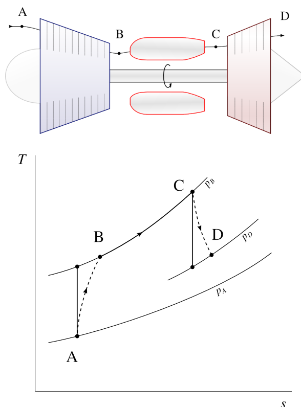
Figure 10.16: A “gas generator” (schematic drawing and temperature-entropy diagram). This machine has no interest in itself but has many derived applications. One of them is the turbocharger , for which a piston engine acts as the combustion chamber, as described in §10.3.5.
