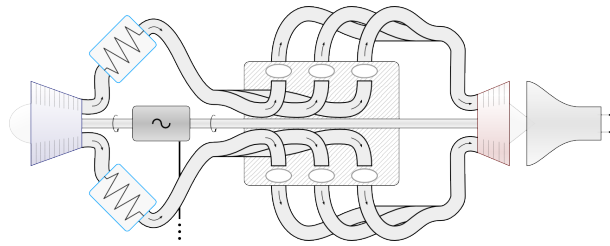
Figure 10.30: Thermodynamic circuit of the air in a 2014 Formula 1 engine. The shaft of the compressor (left) is not connected to the six-cylinder engine (center block) or the car's wheels. However, an electric motor/generator (named MGU-H) allows for extraction or addition of electrical energy. During high power phases, the power of the turbine (right) is in surplus and can be used to charge on-board batteries or drive the wheels with an electric motor. During low power phases, the turbine power is in deficit and the turbo can be driven by the generator to maintain the compression ratio and increase responsiveness.
