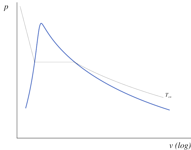
Figure 5.9: Pressure-volume diagram of water, represented with a constant temperature (isothermal) process. The saturation curve is represented in blue.
