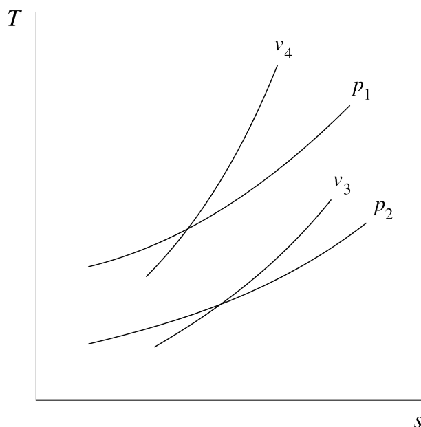
Figure 8.7: Isobaric and isochoric curves on a T - s diagram, for an ideal gas. Here p_1 > p_2 and v_3 > v_4 .
