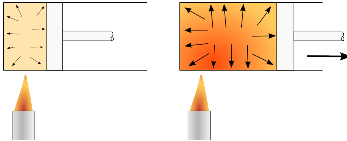
Figure 2.2: Operating principle of an engine. When heat is supplied to a fluid in a closed reservoir, it increases the forces it exerts on the walls of the reservoir. By allowing the reservoir to deform, we let the fluid perform work.
