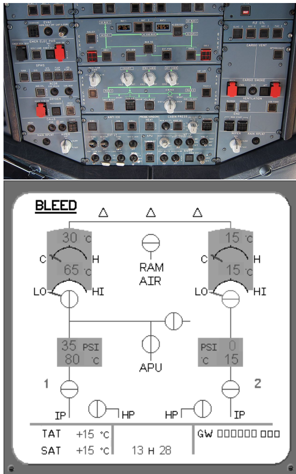
Figure 6.28: Control interface of the ECS in the center of the upper panel of the cockpit of an Airbus A320 and the corresponding EFIS display panel.
