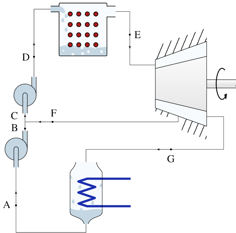
Figure 9.20: Diagram of a steam power plant with steam bleed. The steam prematurely extracted from the turbine is used to heat the liquid water during pumping.
