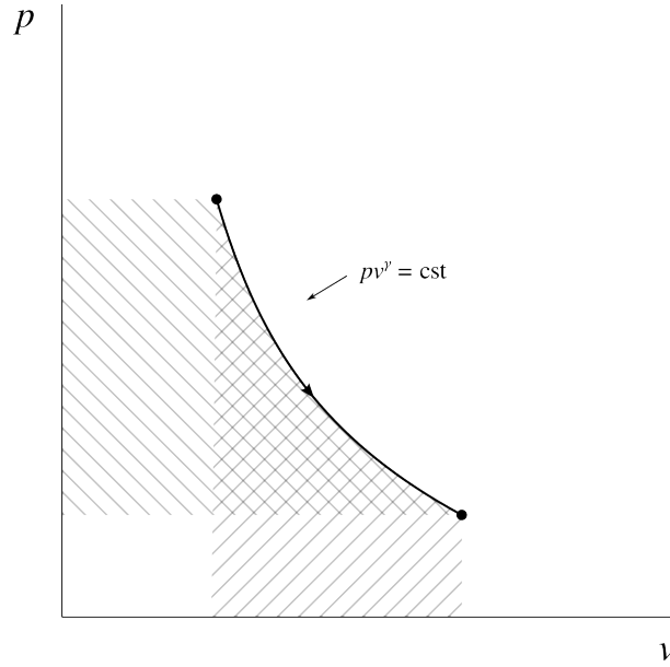
Figure 4.13: Reversible adiabatic expansion of an ideal gas, represented on a pressure-volume diagram.
