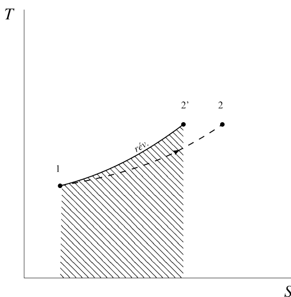
Figure 8.3: Temperature-entropy diagram. During a reversible process, the area under the curve of a T - s diagram represents the transmitted heat Q_{1 \rightarrow 2'} ; but not when it is irreversible. Diagram CC-0 Olivier Cleynen
