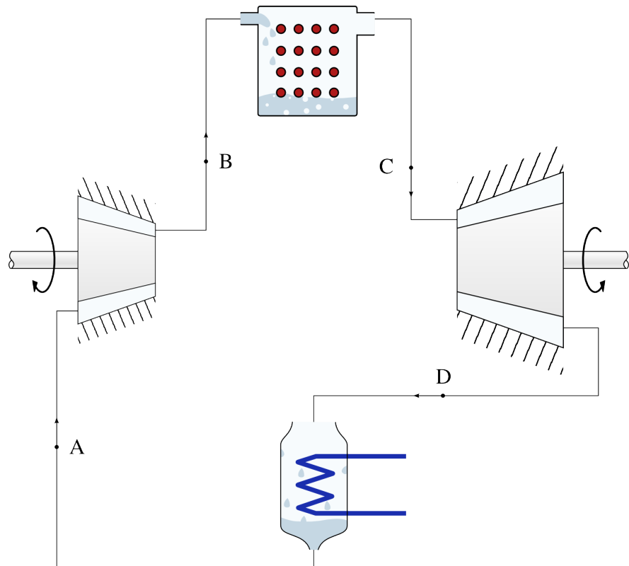
Figure 9.10: Diagram of a steam power plant operating on a Carnot cycle.
