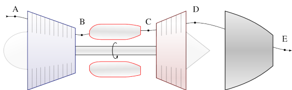
Figure 4.19: Schematic of a turbojet engine. Air flows through the machine from left to right.
