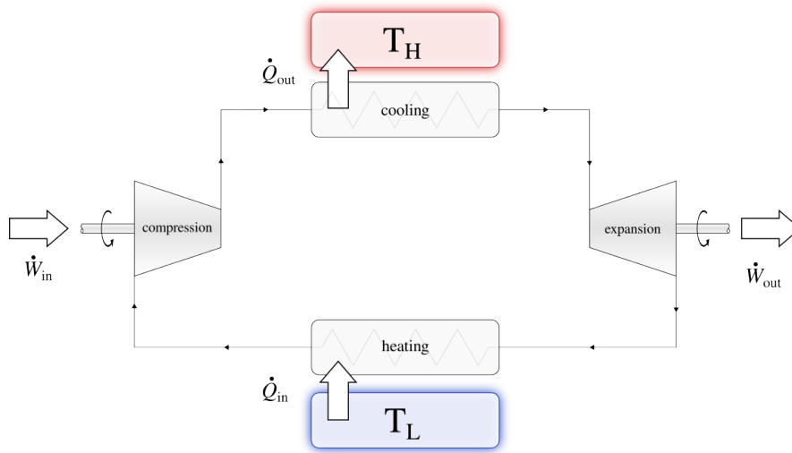
Figure 6.5: A refrigeration cycle, for use in refrigerators, air conditioners, and heat pumps.
