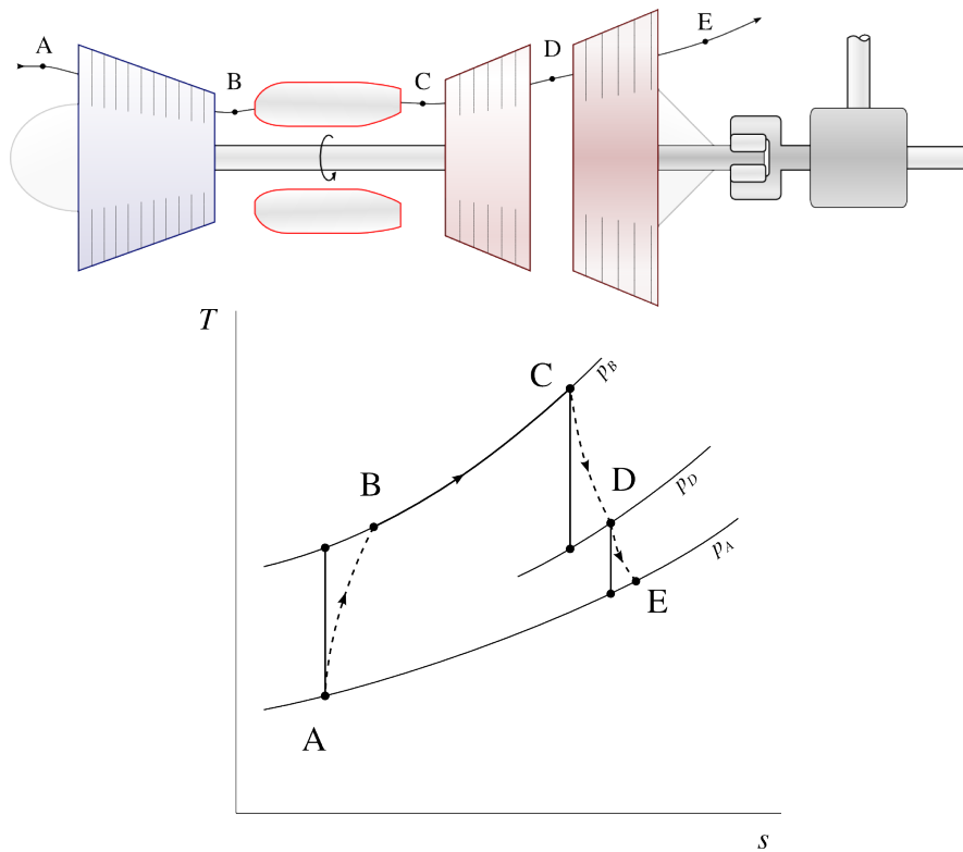
Figure 10.20: Turboshaft engine with a free turbine (schematic and temperature-entropy diagram). The power supplied by the engine comes exclusively from the free turbine.
