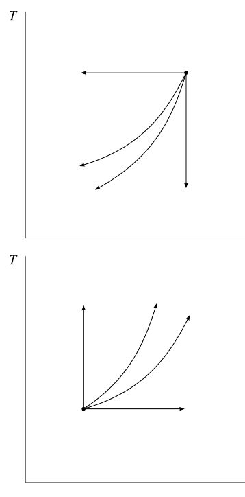
Figure 8.13: Reversible elementary processes of an ideal gas, represented on a temperature-entropy diagram.
