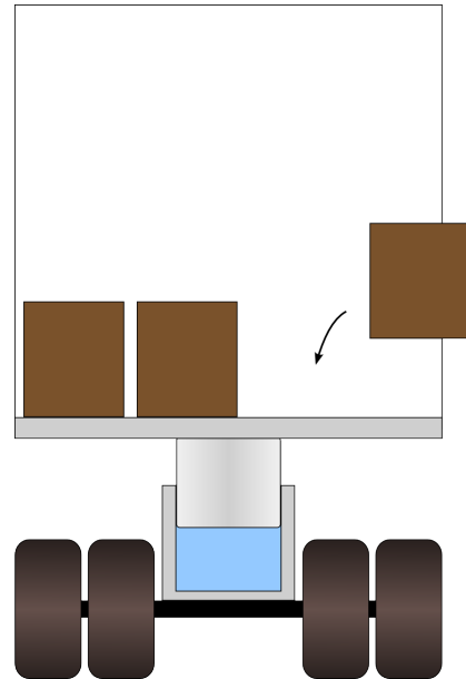
Figure 2.19: Schematic modeling of a truck pneumatic suspension system. The piston, at the center, compresses a mass of air (in blue) when the trailer is loaded.
