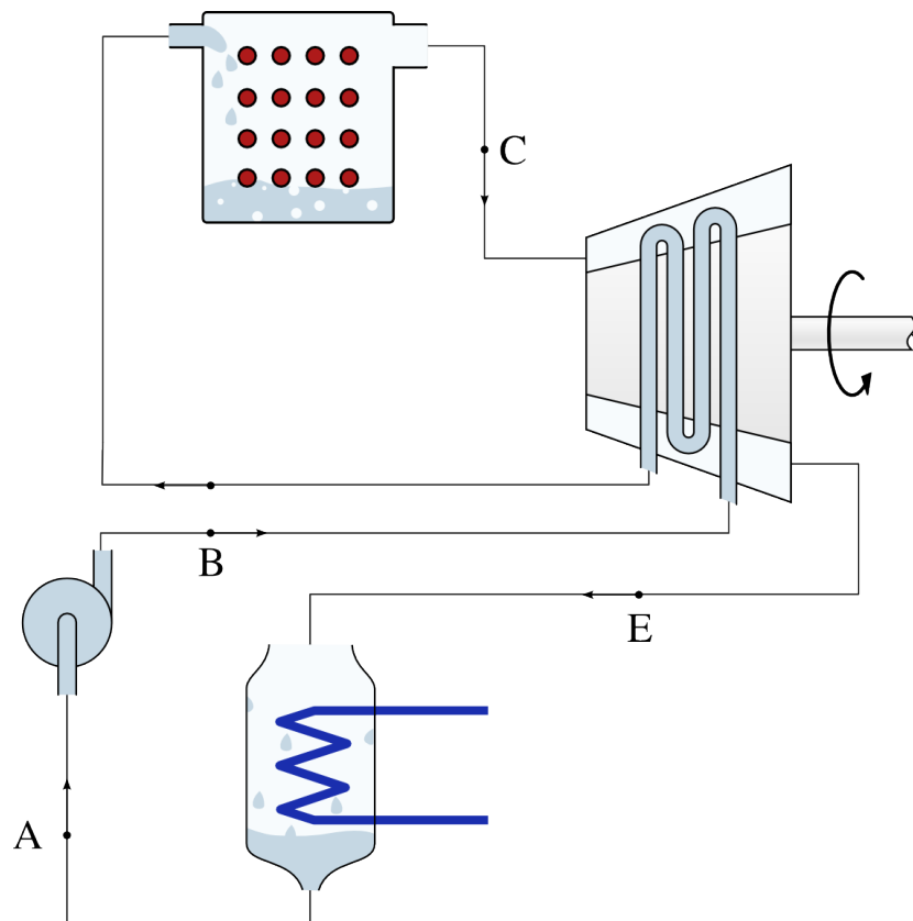
Figure 9.18: Diagram of a steam power plant with regeneration. Heat is extracted from the turbine to heat the liquid water before it enters the boiler. Ideally, heat transfer is reversible.
