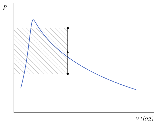
Figure 5.17: Heating at constant volume of a liquid-vapor, represented on a pressure-volume diagram.
