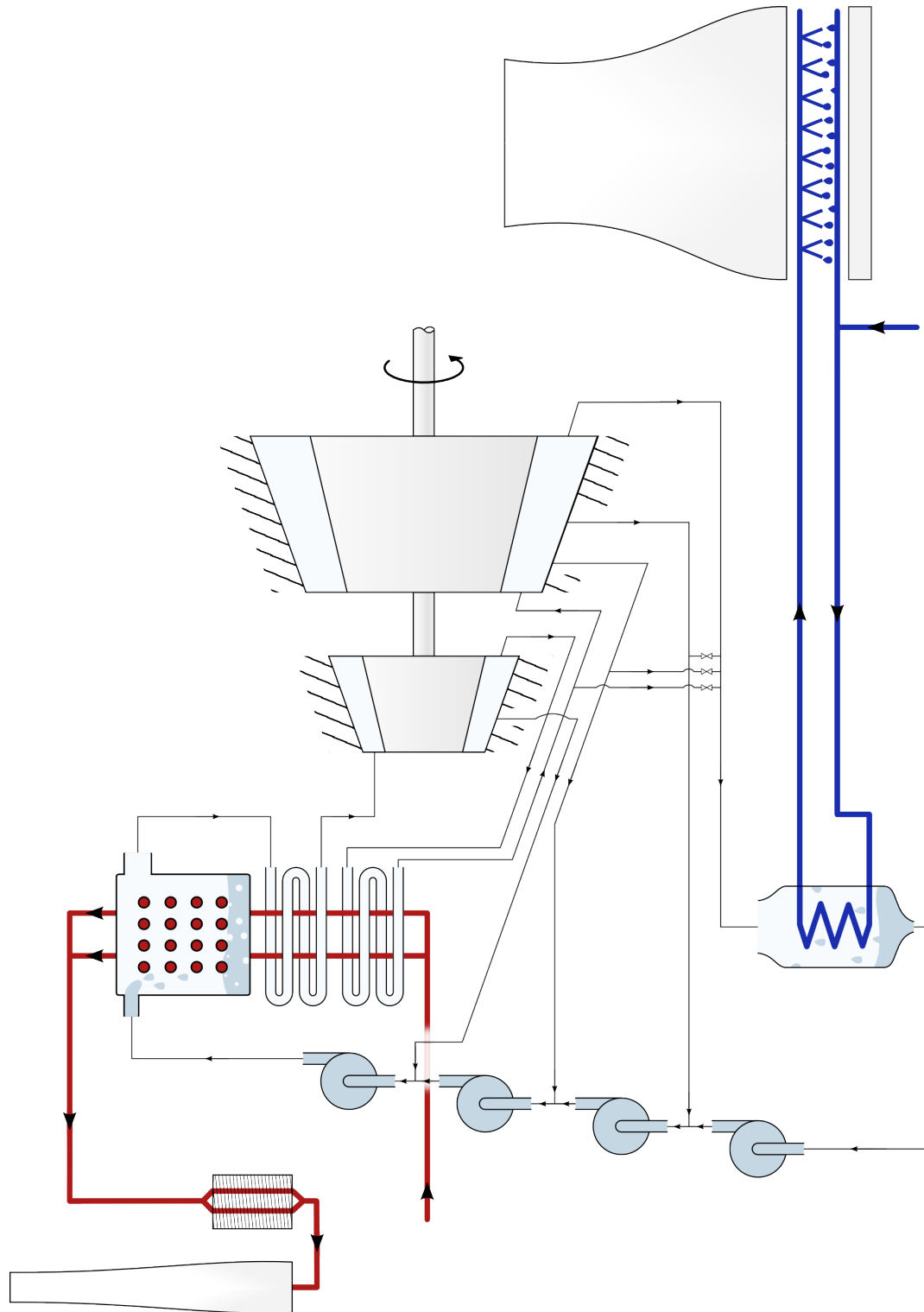
Figure 9.22: A steam power plant circuit combining superheating, reheat, regeneration, and discharge ducts. It is left to the curious student the pleasure of tracing the processes on a temperature-entropy diagram, and imagining themselves at the controls of the machine supplying their coffee maker with electricity.
