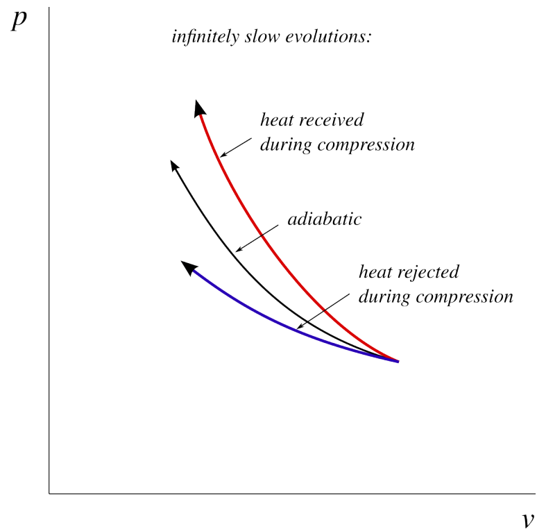
Figure 2.10: Behavior of a fluid when infinitely slowly compressed. The more heat is supplied during compression, the more rapidly the pressure increases. The adiabatic curve represents the case where no heat transfer occurs ( Q = 0 ).
