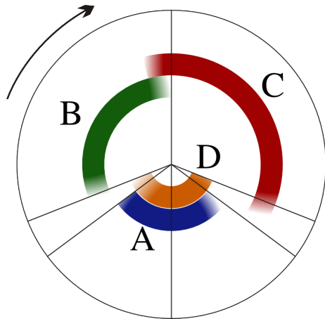
Figure 6.15: Cycle of a two-stroke engine. The four necessary steps for operation are carried out in a single revolution of the crankshaft, that is, two piston movements. Intake (A) occurs during the passage at bottom dead center, compression (B) starts late, and expansion (C) is interrupted to allow scavenging (D) when the piston approaches bottom dead center again.
