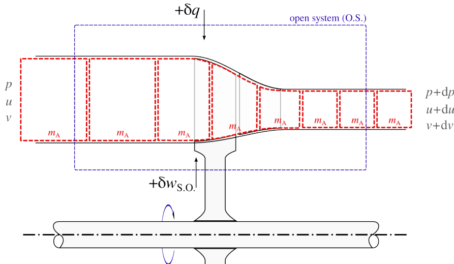
Figure 3.5: The same flow as in figure 3.4, now observed from the viewpoint of a stationary open system crossed from left to right by a steady flow. We seek to quantify the work \delta w_{O.S.} to be supplied to the system so that each mass quantity m_A receives work \delta w_{m_A} .
