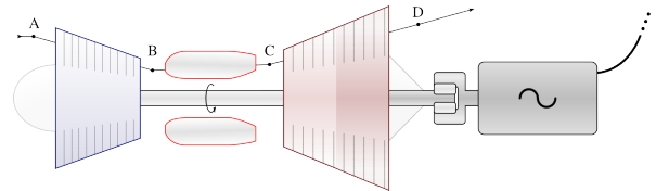
Figure 6.21: A static gas turbine engine, in this configuration named turboshaft , powering an electric generator. The gas is typically expanded (in the turbine, between C and D) to atmospheric pressure.
