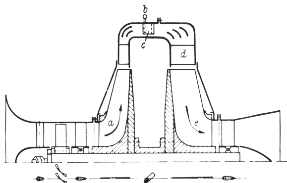
Figure 9.25: Cross-sectional diagram of the Heinkel He S-1 , the first prototype tested by Hans von Ohain in 1937. The compressor consists of an axial stage and a centrifugal stage; the turbine is centripetal. There is only one moving part and its speed is invariant.
