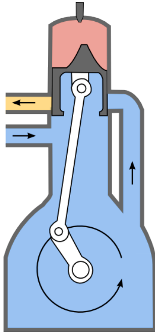
Figure 6.18: Crankcase intake system. The intake air, laden with fuel for combustion and oil for lubricating mechanical parts, first enters the crankcase. It is compressed and then inserted into the cylinder with the sole downward movement of the piston. There is no need for any valve or flap.
