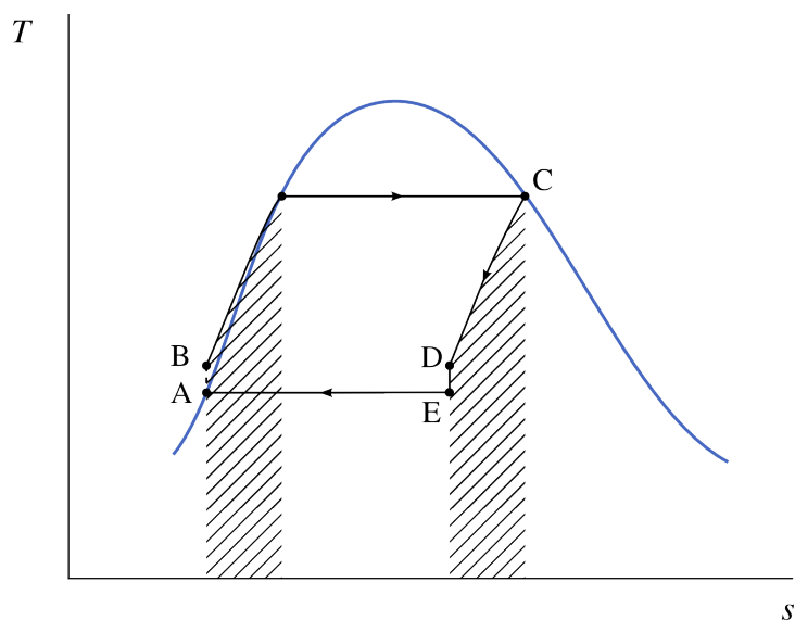
Figure 9.19: Temperature-entropy diagram of a steam power plant with regeneration.
