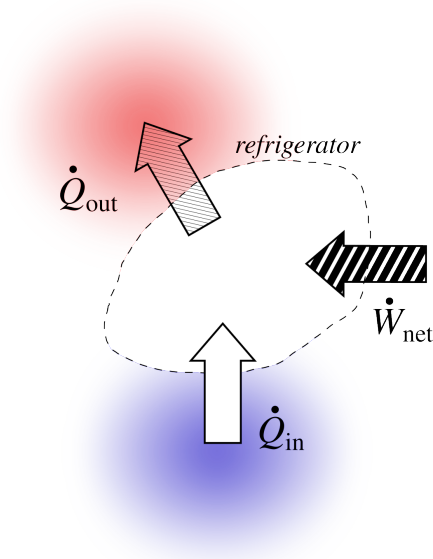
Figure 6.12: Energy transfers associated with a refrigerator or an air conditioner. We aim to obtain a large transfer \dot{Q}_{\text{in}} (result) from the transfer \dot{W}_{\text{net}} (cost).
