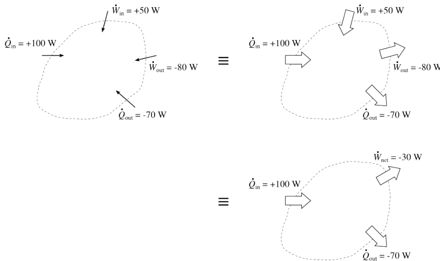
Figure 6.1: New graphical and notation conventions for energy transfers. The white arrows are oriented according to the physical direction of the transfers; The algebraic sum of all the work received and carried out is represented by a single transfer named net work .
