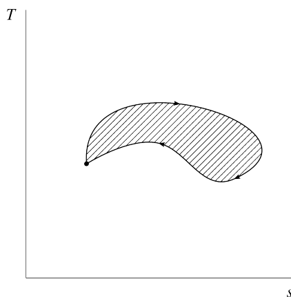
Figure 8.5: Thermodynamic cycle during which heat has been absorbed, and therefore transformed into work. When the path is reversed, heat is rejected (and work absorbed) by the fluid.
