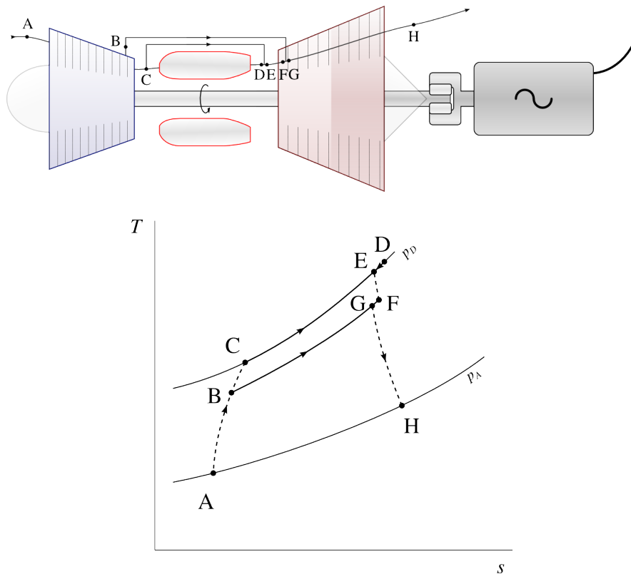
Figure 10.25: Turbine cooling using air taken from the compressor (schematic and temperature-entropy diagram). This air, at moderate temperature, bypasses the combustion chamber and never comes into contact with the fuel. Here the represented engine is a turboshaft, but turbine cooling can be used in any configuration.
