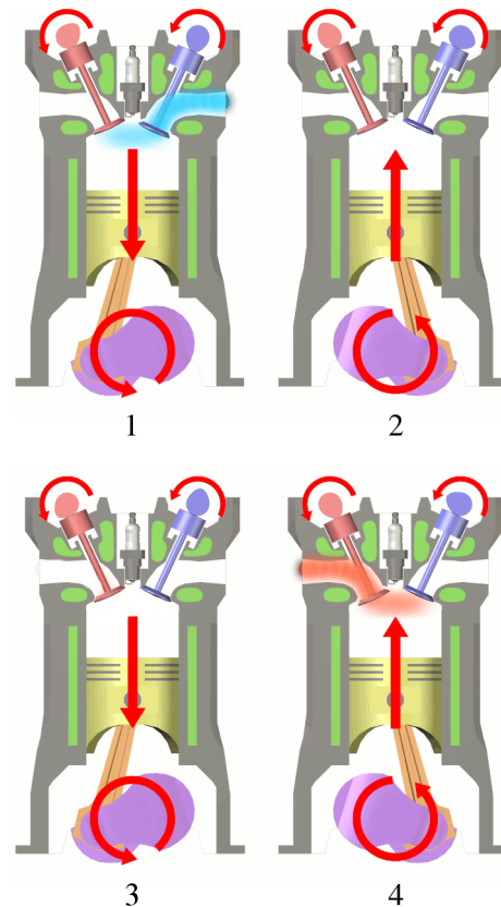
Figure 6.14: The four steps of a four-stroke engine. The piston descends to admit fresh air coming from the right (intake stroke, 1); it then rises to increase the air temperature (compression stroke, 2); useful work production occurs during a descent (power stroke, 3); finally, the air is expelled to the outside during a fourth and last movement (exhaust stroke, 4) before starting the cycle again. Most current piston-cylinder engines follow this process.
