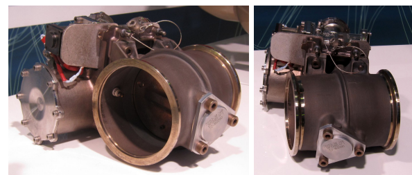
Figure 6.25: Airflow regulation valve of an ECS intended for a Comac C919.
