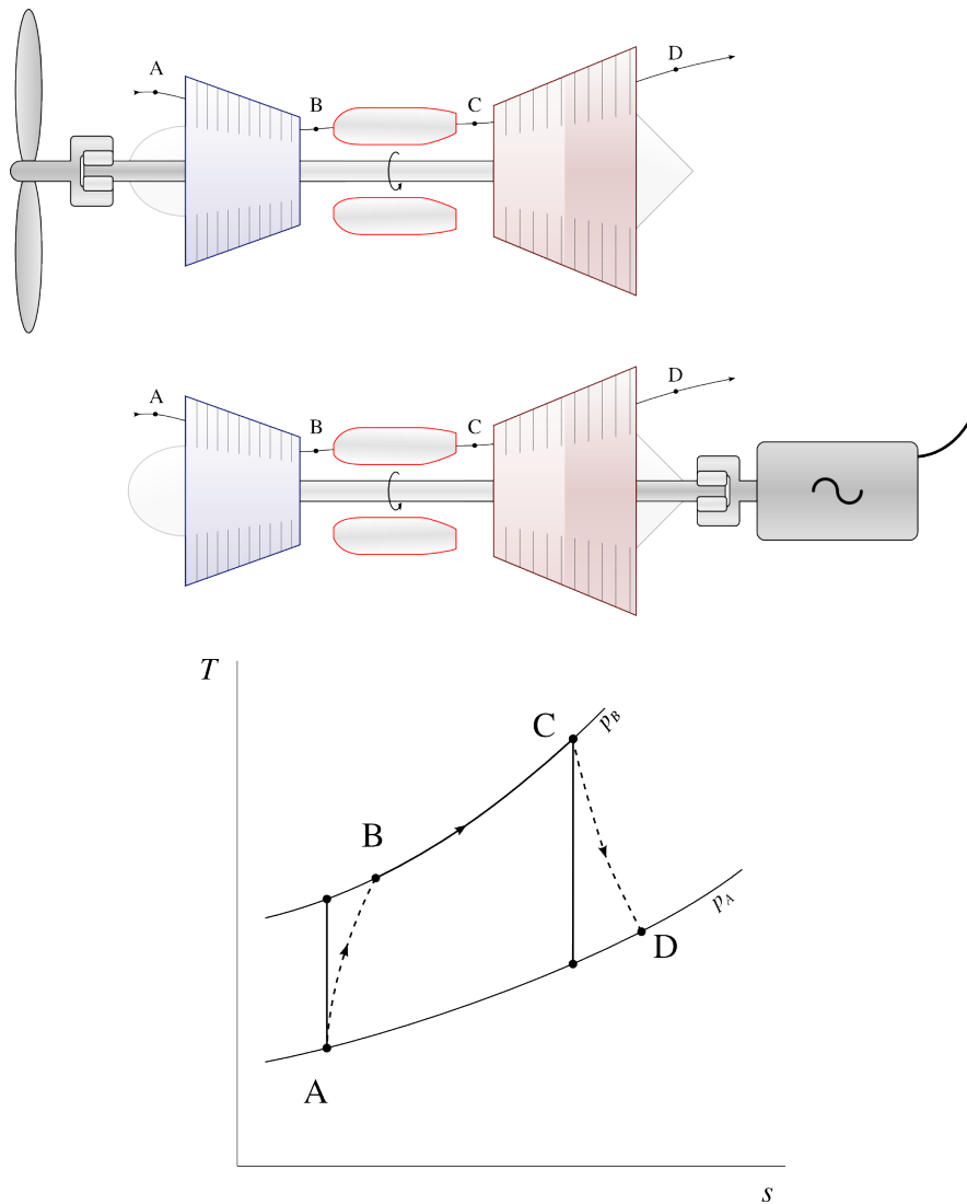
Figure 10.18: Schematics and temperature-entropy diagram of a turboprop (top) and a turboshaft engine (bottom). The power extracted by the turbine exceeds that absorbed by the compressor and is used to power the propeller or a generator.
