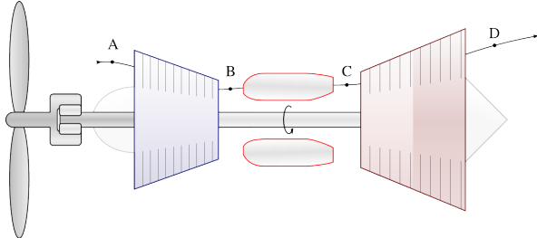
Figure 3.17: Schematic diagram of a turboprop engine. These engines are studied in more detail in §10.5.4 p. 286.
