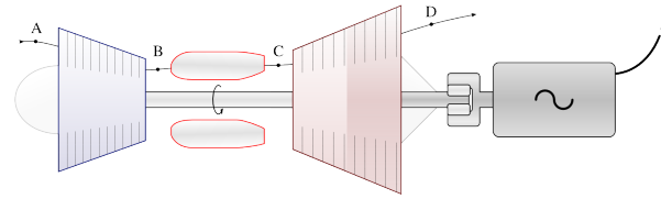
Figure 3.11: Schematic diagram of an electricity-generating turboshaft engine
