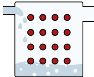
Figure 9.4: Schematic representation of a fire-tube boiler. Water enters in the liquid state on the left and exits at the top right in the form of saturated steam. In fire-tube boilers , the gas pipes pass through the heat exchanger filled with water. In more recent water-tube boilers , it is the water pipes that pass through the heat exchanger filled with hot gases. The latter technique is not detailed in this book, but its thermodynamic working principle is identical.
