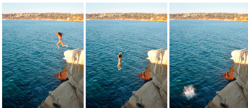
Figure 8.1: We have the intuition and an inner conviction that these three photos were taken in a very particular order. A calculation of the entropy in these three situations, in which the energy is the same, allows us to determine this order by associating a calculable quantity with our intuition.
