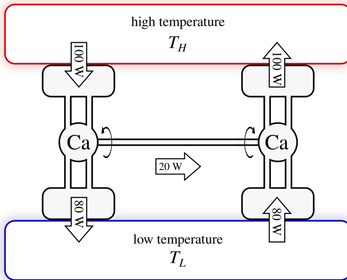
Figure 7.6: Two Carnot machines, an engine (left) and a refrigerator (right). The first powers the second, and since they are reversible (in the thermodynamic sense of the word), the heat flows are balanced.
