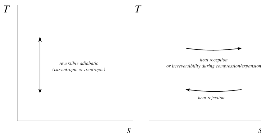
Figure 8.4: elementary processes on temperature-entropy diagrams.
