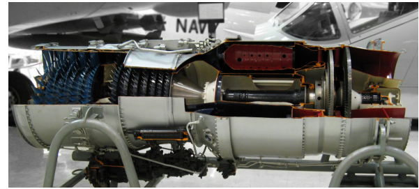
Figure 10.35: A turbojet with twin spools Pratt & Whitney J52 (or JT8A), built in 4500 units. It still equips the EA-6B Prowler.
