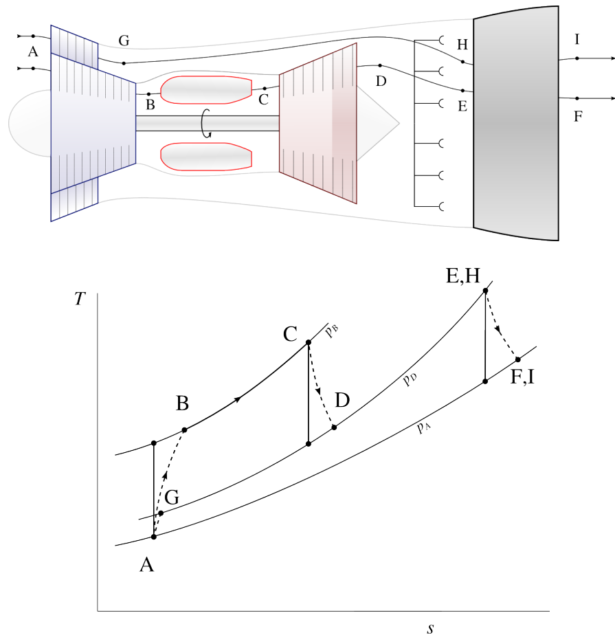
Figure 10.24: Afterburner on a dual-flow turbojet engine (schematic and temperature-entropy diagram). States E and H are not necessarily merged in practice.
