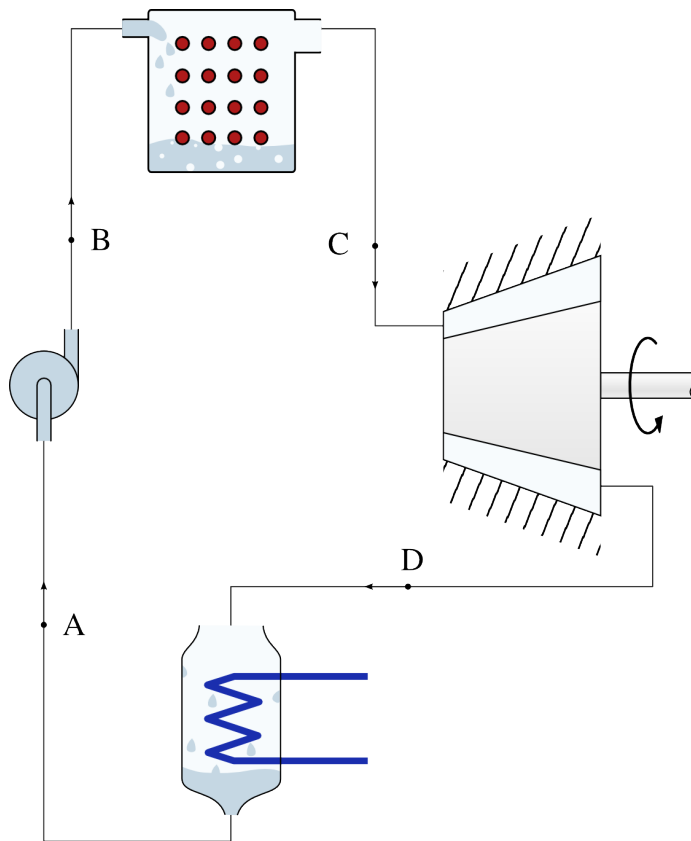
Figure 9.12: Diagram of a steam power plant operating on a Rankine cycle. The water at the outlet of the condenser is in the form of saturated liquid; it enters the boiler at a lower temperature.
