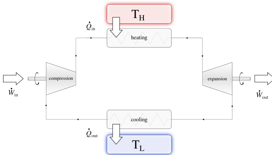
Figure 6.2: Engine thermodynamic cycle. The fluid absorbs heat supplied at high temperature T_H . The compression power is lower than the expansion power: the net power in the form of work \dot{W}_{net} = \dot{W}_{in} + \dot{W}_{out} is negative.
