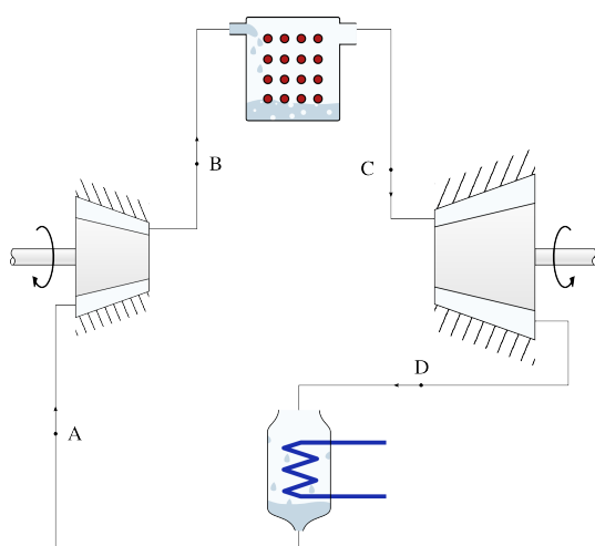
Figure 7.17: Schematic representation of a steam power plant operating with the Carnot cycle.
