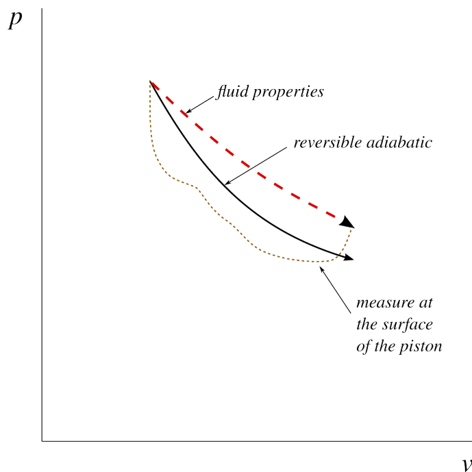
Figure 2.15: Irreversible adiabatic expansion on a pressure-volume diagram. The work received by the piston is less than it would have been with a slow motion. The path followed by the fluid is represented with dashes, because the pressure is not homogeneous during the movement.
