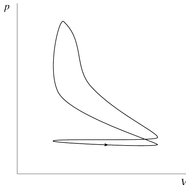
Figure 10.5: A realistic representation of the pressure and volume changes during a cycle in a practical gasoline engine.
