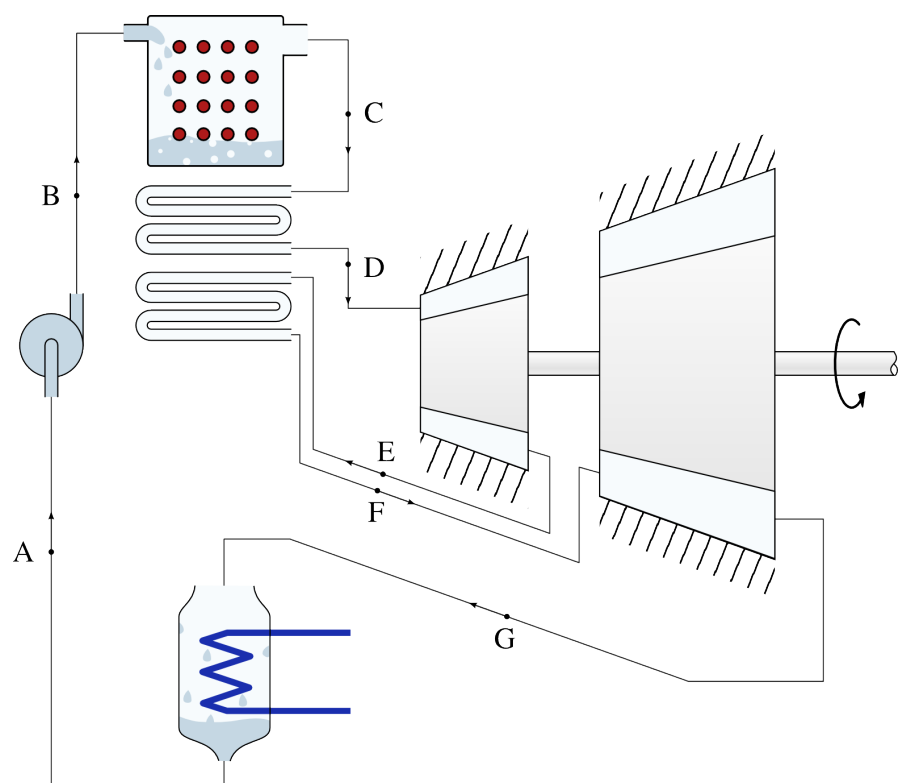
Figure 9.16: Diagram of a steam power plant operating on a reheated Rankine cycle.
