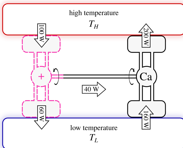
Figure 7.7: Proof by contradiction that the best possible engine is reversible. A hypothetical engine (on the left) with higher efficiency than a reversible refrigerator (on the right) could simply power the latter. Thus, we would obtain a spontaneous net heat flow (here of 100 W) from the cold source to the hot source, without a net input of work: according to the second law, this is impossible.
