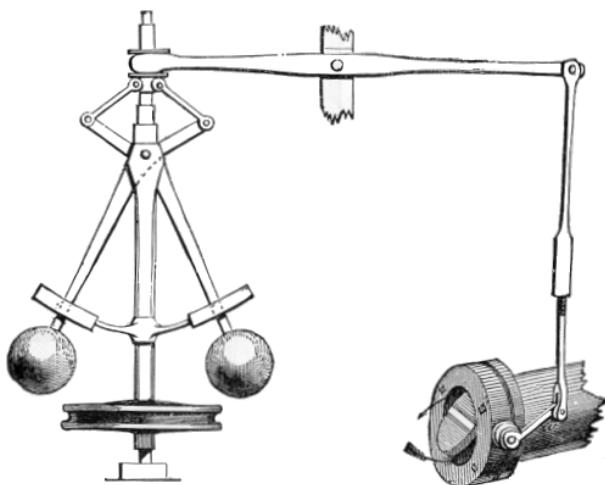
Figure 5.25: The ball governor, a mechanism originating from windmills and integrated into steam engines by James Watt.
