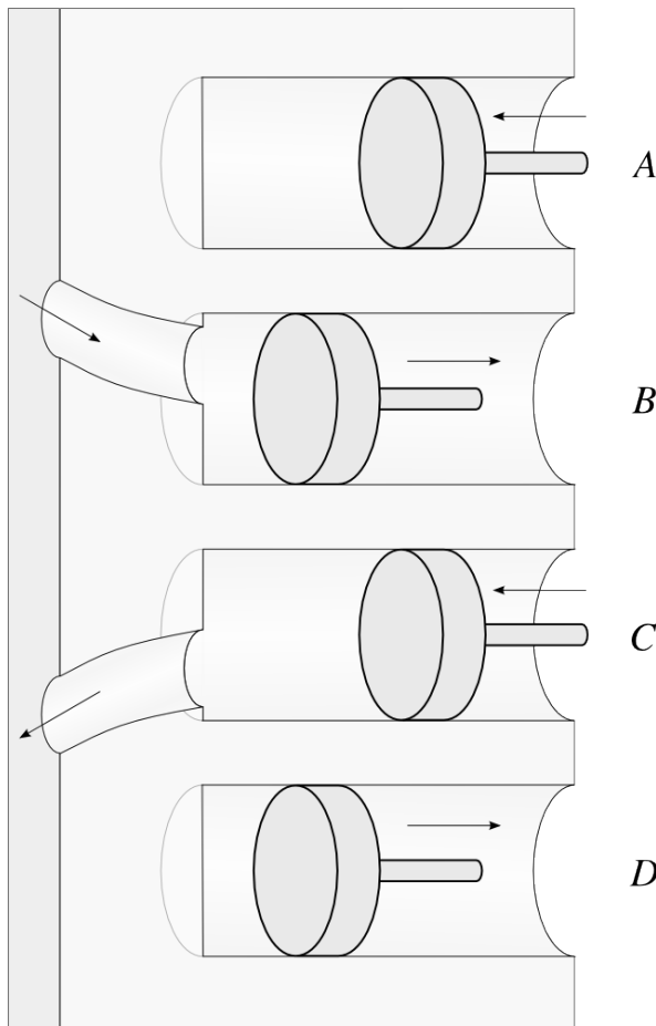
Figure 2.22: Schematic representation of the operation of a four-cylinder engine. Pistons A and C are going up, and pistons B and D are going down. They are all connected to the same motor shaft, not shown here.
