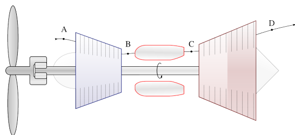
Figure 10.33: Internal arrangement of a turboprop.
