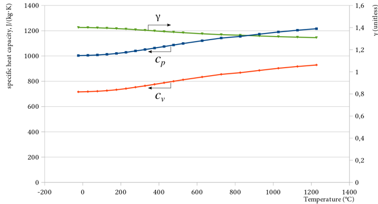
Figure 4.4: Specific thermal capacity of air as a function of temperature. There is a noticeable change in values in the temperature range used in engineering, which we will neglect in the scope of this book.
