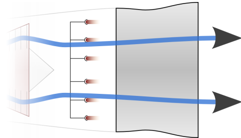
Figure 3.16: Schematic diagram of an afterburner system. Its operation is studied in §10.6.2 p. 291.
