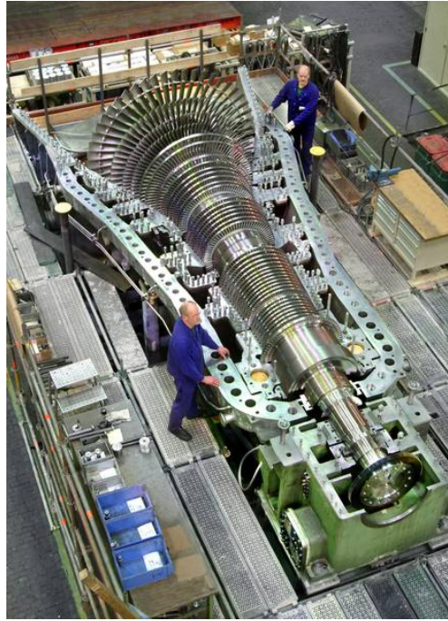
Figure 9.5: Turbine of a medium-sized steam power plant. As the water passes through the turbine, it loses energy in the form of work and its specific volume increases, requiring increasingly larger blades.
