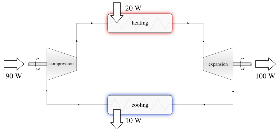
Figure 10.1: The cycle of a hypothetical engine with low work ratio. The delivered power is \dot{W}_{\text{net}} = \dot{W}_{\text{compression}} + \dot{W}_{\text{expansion}} = +90 + (-100) = -10 \text{ W} , and the efficiency \eta_{\text{engine}} = -\frac{\dot{W}_{\text{net}}}{\dot{Q}_{\text{in}}} = -\frac{-10}{20} = 50 \text{ \%} .
