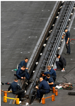
Figure 5.32: Cylinder of a steam catapult from the USS Abraham Lincoln Photo by Geoffrey Lewis, U.S. Navy (public domain)
