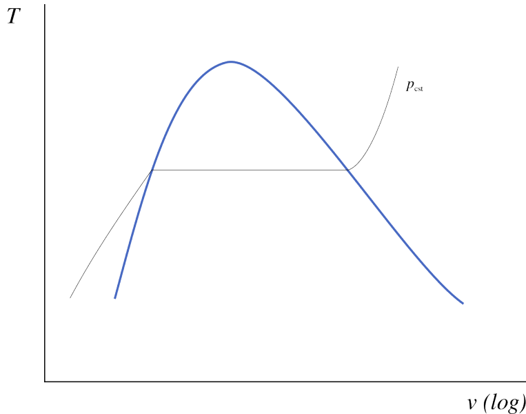
Figure 5.7: Temperature-volume diagram of water, represented with a constant pressure (isobaric) process. The saturation curve is represented in blue.
