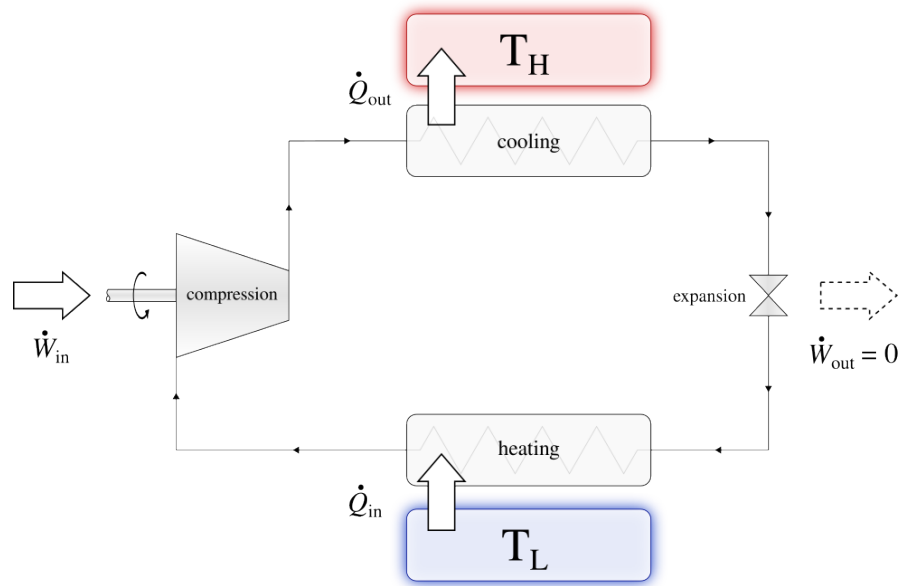
Figure 6.7: A modified refrigeration cycle using a throttling valve. When using liquids/vapors, it is possible to avoid extracting work during expansion. The use of a simple valve is sufficient to lower the temperature of the fluid.
