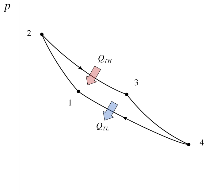
Figure 7.10: Pressure-volume diagram of the Carnot engine performed with a perfect gas. The processes 2 \rightarrow 3 and 4 \rightarrow 1 are done at T_H and T_L , respectively.
