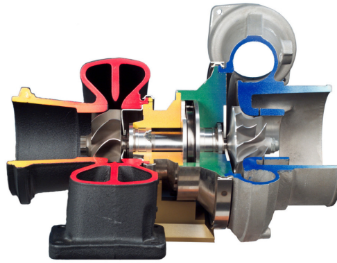
Figure 10.7: A cutaway view of a turbo to show its internal arrangement. Atmospheric air enters from the right and is compressed as it is propelled outward by the centrifugal compressor; it is then fed into the engine. Exhaust gases enter from the center left and exit to the left after spinning the centripetal turbine, which powers the compressor via the central rotating shaft. Since the only moving part is very compact (about 20 cm here), very high rotation speeds can be achieved, typically exceeding 200 000 rpm.
