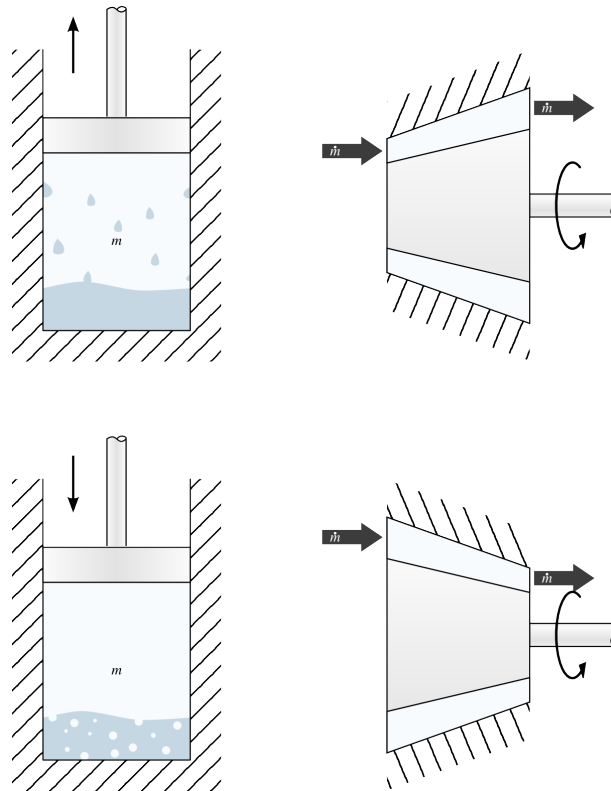
Figure 5.20: A reversible adiabatic (isentropic) process undergone by a liquid-vapor. In a closed system (left) as well as in an open system (right), the enclosure is perfectly insulated, so that there is no heat transfer, even if its temperature varies.
