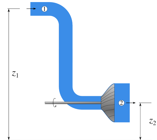
Figure 1.12: Schematic diagram of a water turbine. Water enters at the top left, rotates the turbine blades, is heated by internal friction, and exits at the bottom right of the machine.
