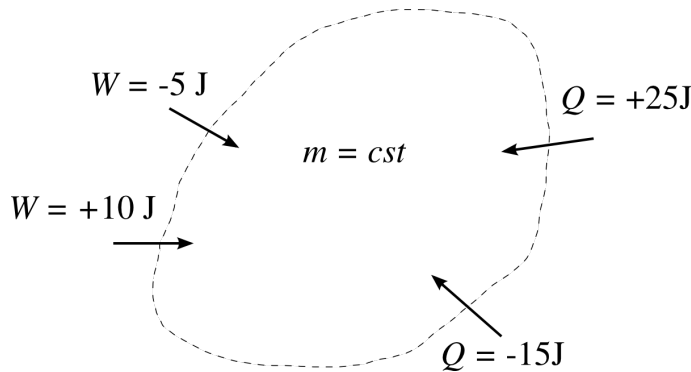
Figure 2.4: Sign conventions for a closed system. Incoming flows are positive, outgoing flows are negative; they are all represented with inward-pointing arrows. The mass quantity is constant.
