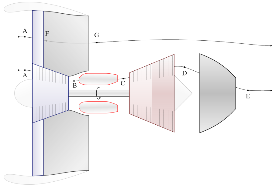
Figure 10.19: Schematic diagram of a turbofan. The engine's thermodynamic core ( A \rightarrow E ) mechanically powers the fan, which allows the bypass flow ( A \rightarrow G ) to provide the majority of the thrust.
