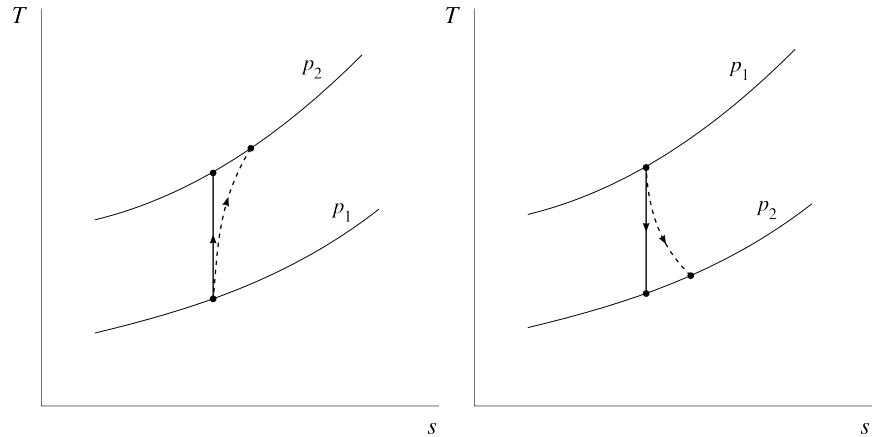
Figure 8.11: Theoretical (isentropic, solid lines) and real (dotted lines) adiabatic expansions and compressions.
