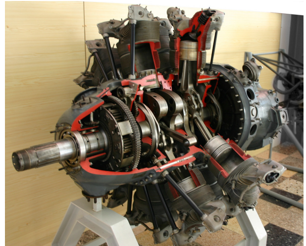
Figure 9.24: Cross-section of a Pratt & Whitney Twin Wasp engine (1932), showing the internal arrangement with connecting rods and crankshafts connecting the two rows of seven pistons arranged in a star pattern. The engine, with a displacement of 30 L, produced over 1000 hp and was produced in over 170 000 units.
