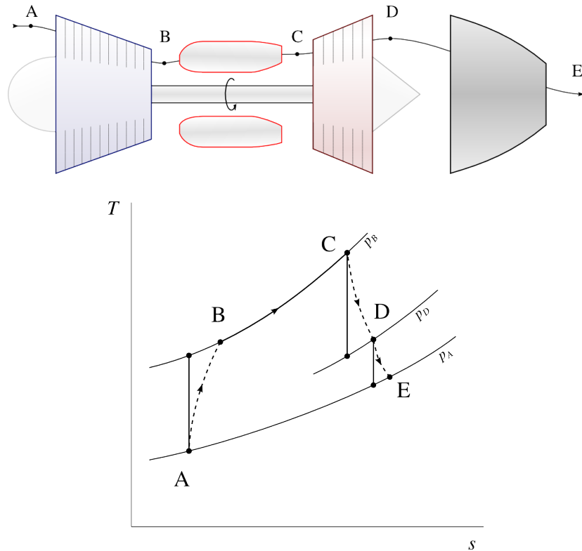
Figure 10.17: Turbojet (schematic and temperature-entropy diagram). At the outlet of the turbine, the air is still pressurized; it is expanded in a nozzle in order to be accelerated.
