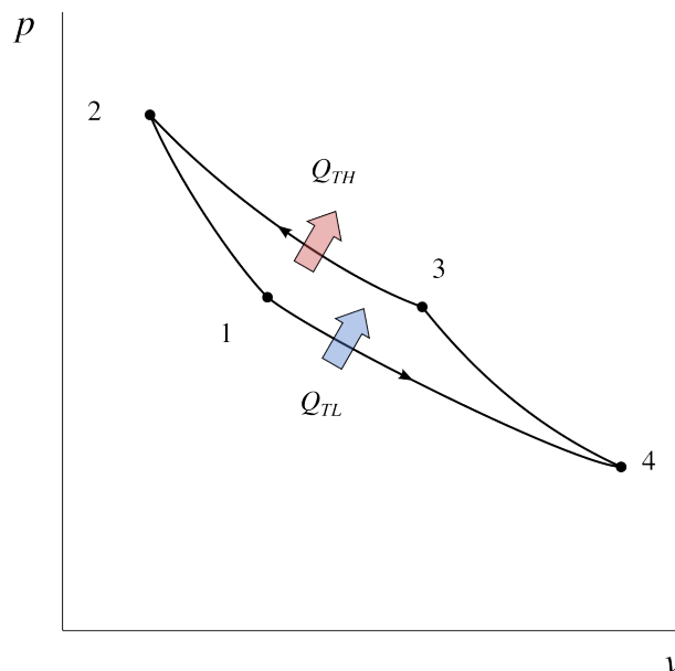
Figure 7.11: Pressure-volume diagram for a reversed Carnot cycle, namely, in refrigeration mode (refrigerator or heat pump), with a perfect gas.
