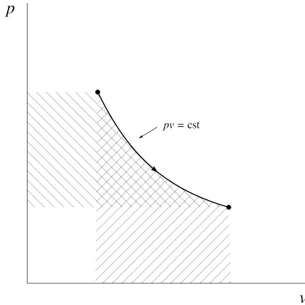
Figure 4.11: Expansion (heating) at constant temperature of an ideal gas, represented on a pressure-volume diagram.
