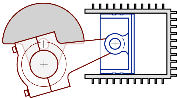
Figure 2.20: Cross-sectional diagram of a small piston air compressor. The intake and exhaust valves are not shown.
