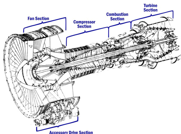
Figure 10.36: Cutaway diagram of a General Electric CF6-6 . The engine propelled all major long-haul aircraft families of the 1970s and 1980s.
