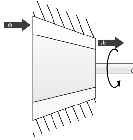
Figure 10.9: Schematic representation of an air compressor.
