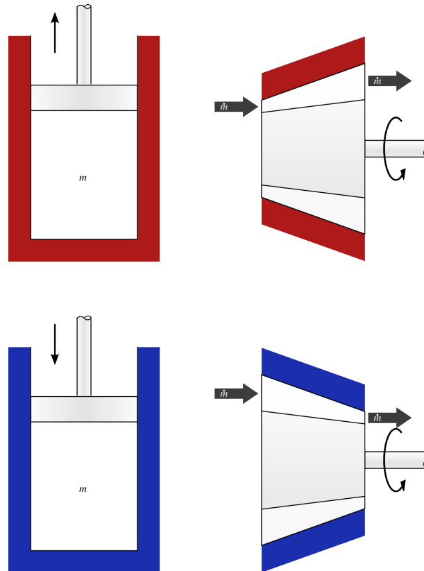
Figure 4.10: A constant-temperature (isothermal) process undergone by an ideal gas. In a closed system (left), the gas is allowed to do work on a piston while being heated, and conversely, work is done on the gas when it is cooled. In an open system (right), the same manipulations are carried out continuously.
