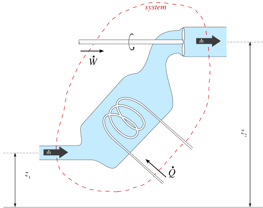
Figure 3.3: An arbitrary open system. The system (whose boundaries are dashed lines, in red) is crossed from left to right by the fluid flowing with a constant mass flow rate \dot{m} . It receives power \dot{W}_{1 \rightarrow 2} in the form of work and power \dot{Q}_{1 \rightarrow 2} in the form of heat.
