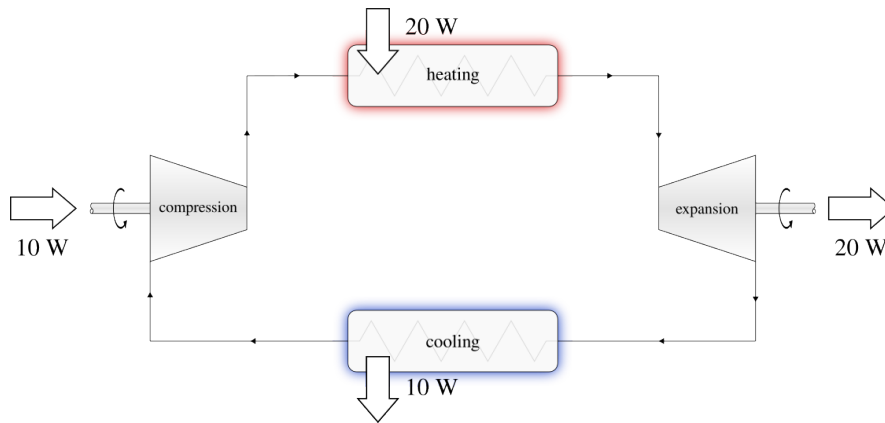
Figure 10.2: The cycle of a second (also hypothetical) engine, with a high work ratio. The delivered power \dot{W}_{\text{net}} = +10 + (-20) = -10 \text{ W} , and the efficiency \eta_{\text{engine}} = -\frac{-10}{20} = 50 \% are identical to those of the engine described in figure 10.1.
