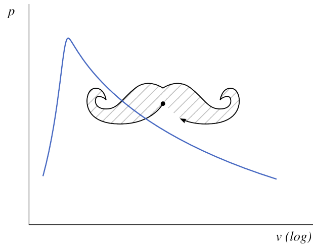
Figure 5.22: A completely arbitrary process undergone by a liquid-vapor represented on a pressure-volume diagram. In addition to a deplorable sense of humor, such a process requires an extremely complex combination of heat and work transfers, which the student is invited to imagine. Diagram CC-0 Olivier Cleynen
