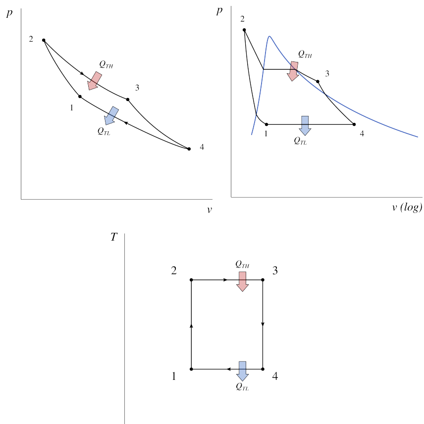
Figure 8.6: Carnot engine cycle, on a p - v diagram for an ideal gas (left), on a p - v diagram for a liquid-vapor system (right), and on a T - s diagram (bottom). Regardless of the fluid used, the temperature-entropy diagram remains the same.
