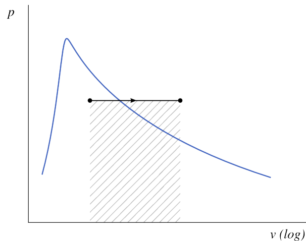
Figure 5.15: Heating at constant pressure of a liquid/vapor, represented on a pressure-volume diagram.
