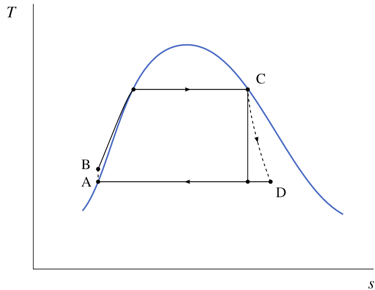
Figure 9.13: Temperature-entropy diagram of a steam power plant operating on a Rankine cycle.
