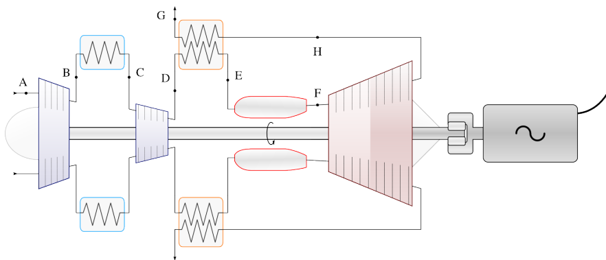
Figure 10.23: Turboshaft generator with an intercooler and an economizer heat exchanger. The exhaust gases are redirected inside the engine to supply heat to the gases at the entrance of the combustion chamber. It is left to the student to determine the limits of the process.
