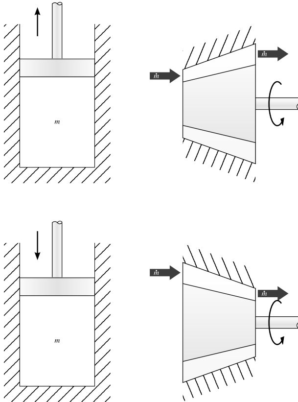
Figure 4.12: A reversible adiabatic (isentropic) process undergone by an ideal gas. In a closed system (left) as well as in an open system (right), the apparatus is perfectly insulated, so that there is no heat transfer, even if the gas temperature varies.
