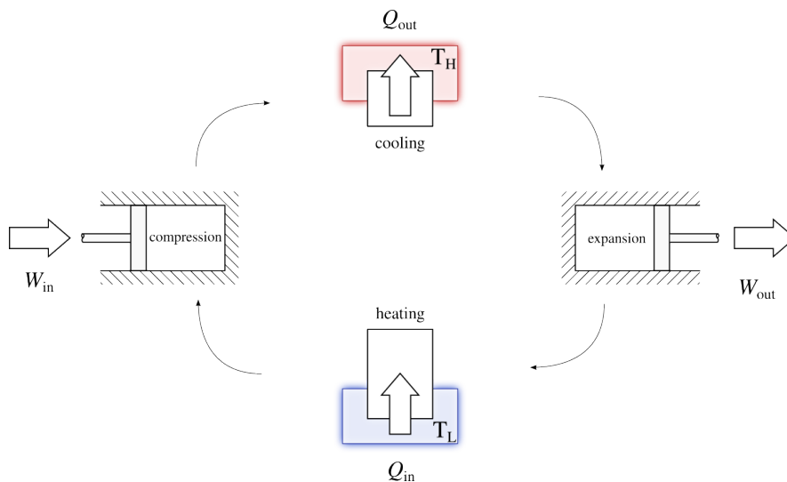
Figure 6.6: A refrigeration cycle carried out by separating the stages in time (rather than in space as shown in figure 6.5)
