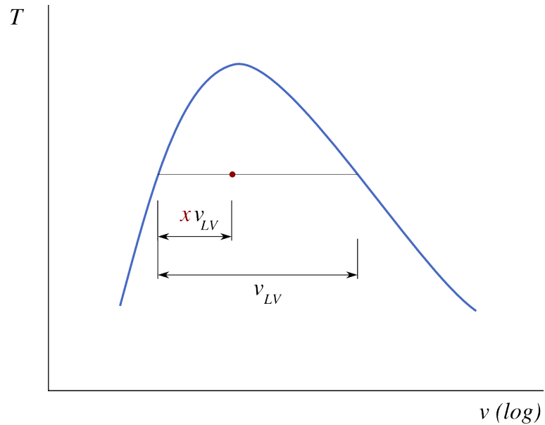
Figure 5.11: The vapor dryness fraction represented by the point position on a T-v diagram.
