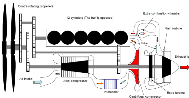
Figure 10.27: Schematic diagram of the thermodynamic circuit of the Napier Nomad I . The shafts of the turboshaft and of the Diesel engine each drove one propeller. However, the two units were mounted in series: the air first passed through the compressors, then through the cylinders, and finally through the turbine(s). The engine power, as was customary in 1950, was controlled using a single mechanical control lever!
