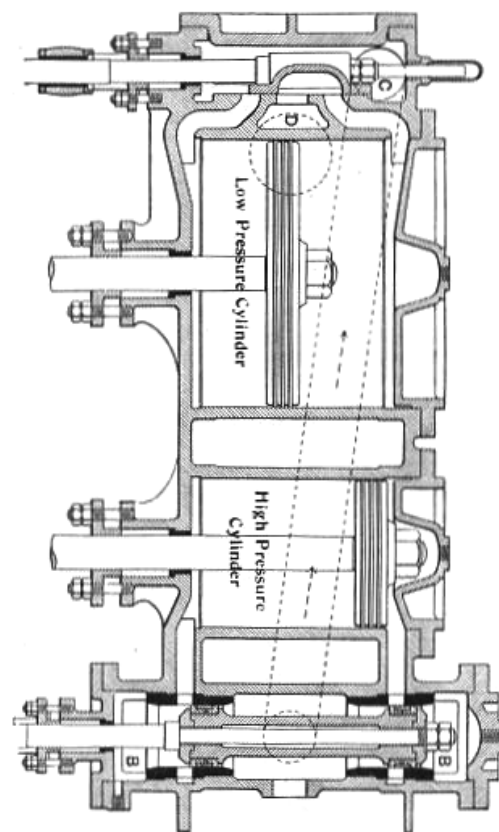
Figure 2.18: Different steam compound systems.
