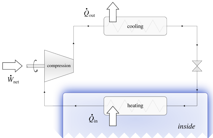
Figure 6.9: Arrangement of a refrigerator or air conditioner. The machine is configured to reject heat outside (where the temperature is higher) which it extracts from the inside (where the temperature is lower). This is exactly the same machine as in figure 6.8.
