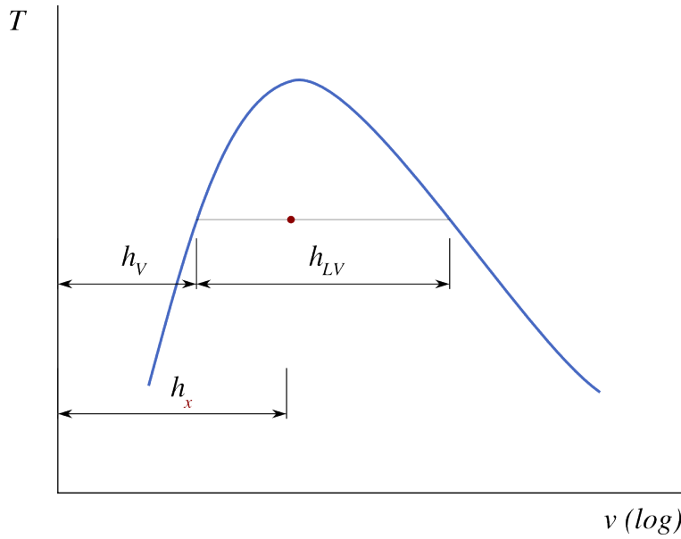
Figure 5.12: Enthalpy h_x of a mixture as a function of the enthalpies in the saturated state and of vaporization.
