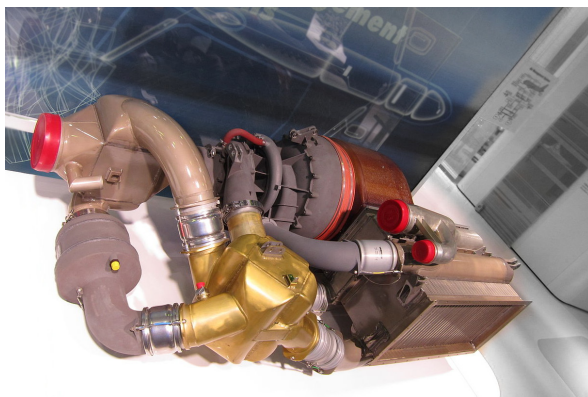
Figure 6.23: A ECS intended for a Comac C919, approximately 1.5 m in length.
