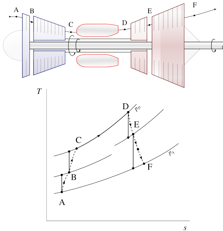
Figure 10.21: Twin-spool turboshaft engine (schematic and temperature-entropy diagram). The two shafts rotate at different speeds.
