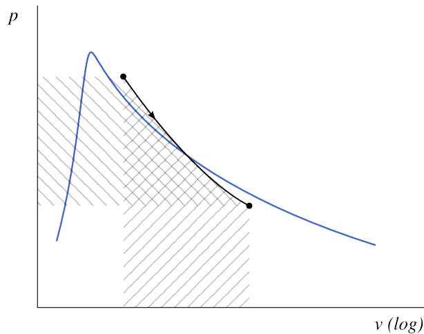
Figure 5.21: Reversible adiabatic expansion of a liquid-vapor, represented on a pressure-volume diagram.
